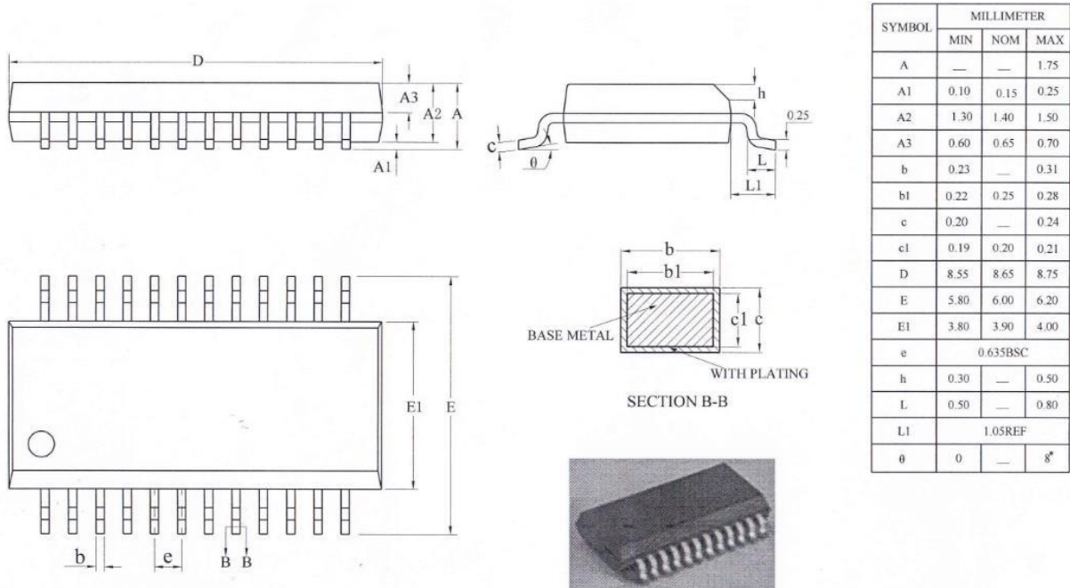
Figure 3-1. AC6965D_QSOP24 Package
