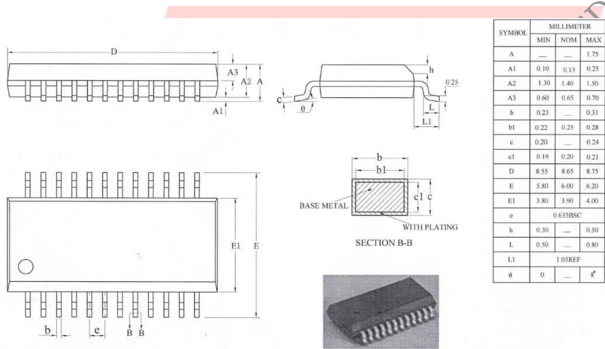
Figure 3-1. AC6965A Package
