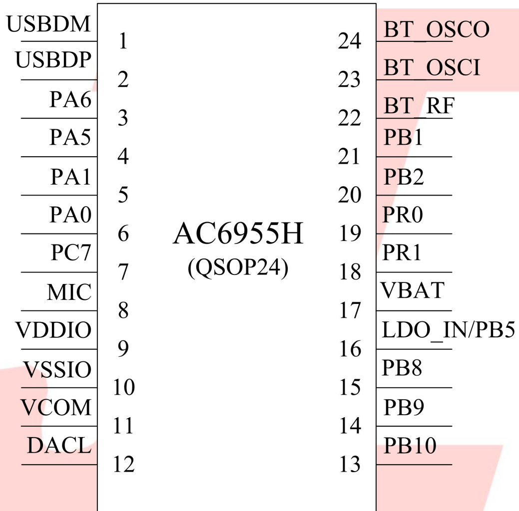
Figure 1-1 AC6955H Package Diagram
