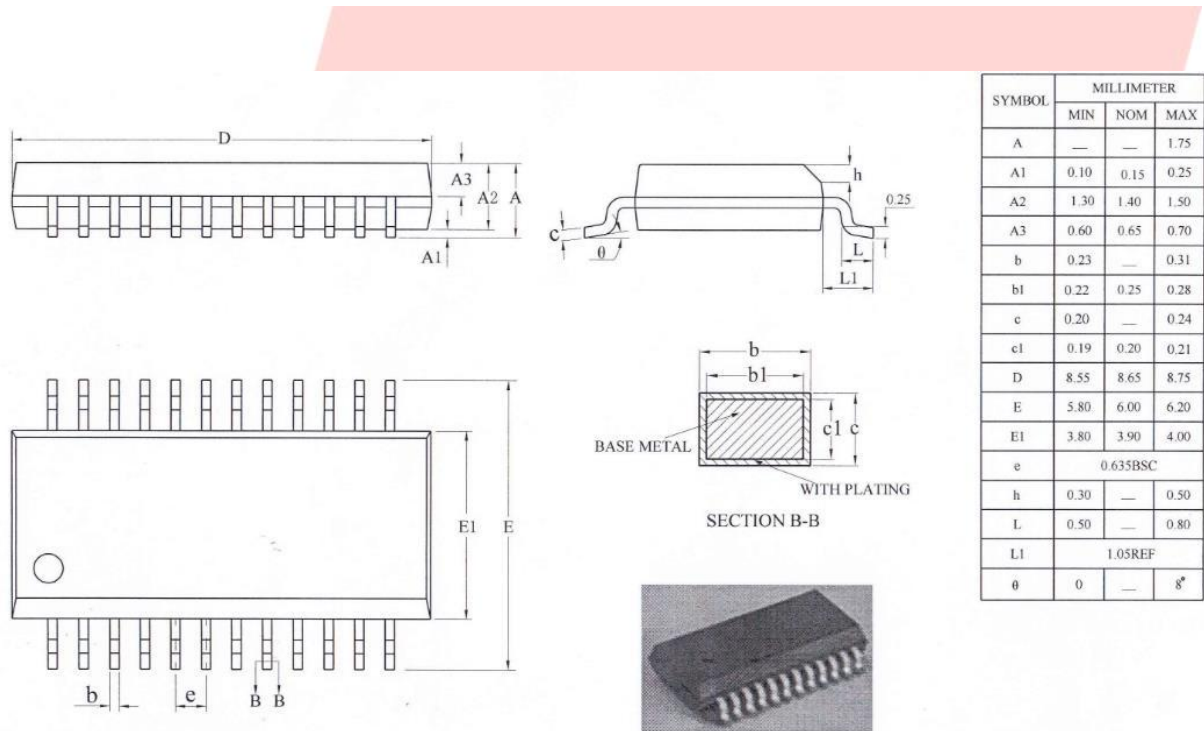
Figure 3-1. AC6955H Package
