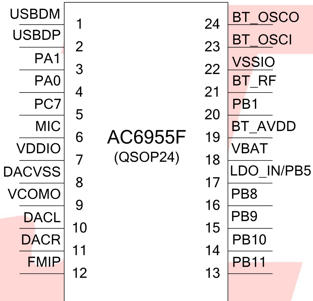
Figure 1-1 AC6955F Package Diagram
