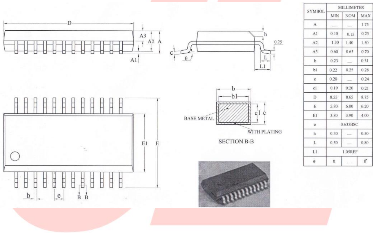
Figure 3-1. AC6955F Package
