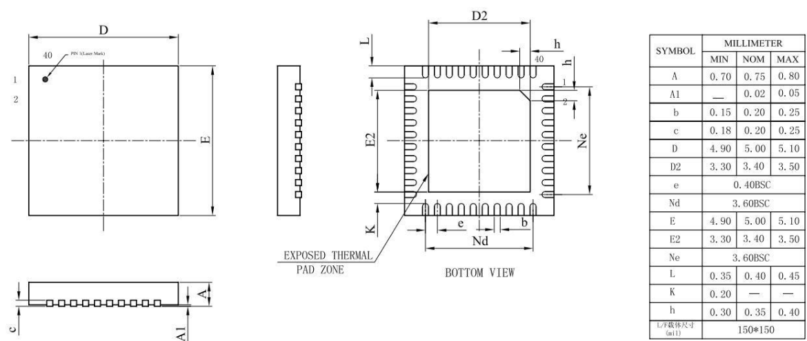
Figure 3-1 AC6958C_QFN40 Package
