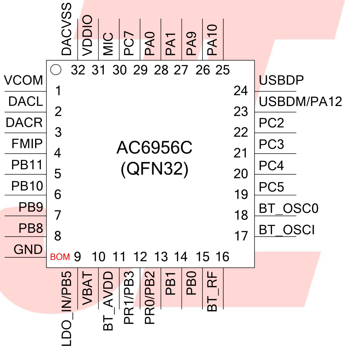
Figure 1-1 AC6956C Package Diagram
