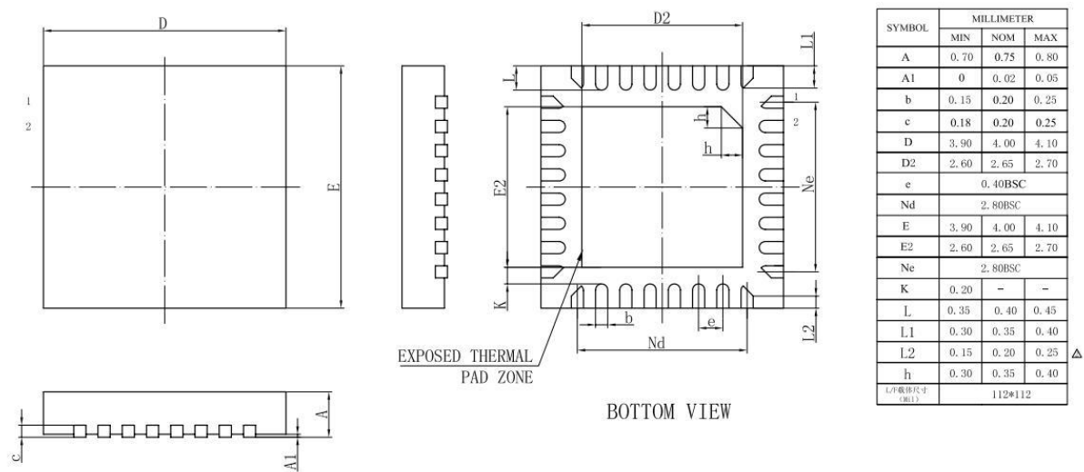
Figure 3-1 AC6956A_QFN32_4x4 Package
