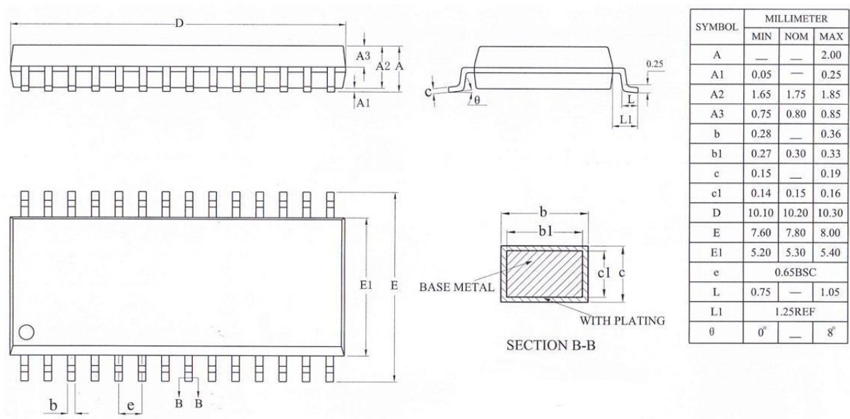
Figure 3-1 AC6952D Package
