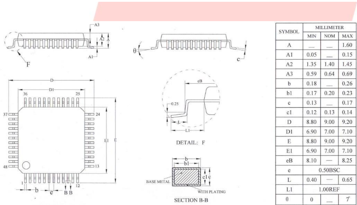
Figure 3-1. AC6951C Package
