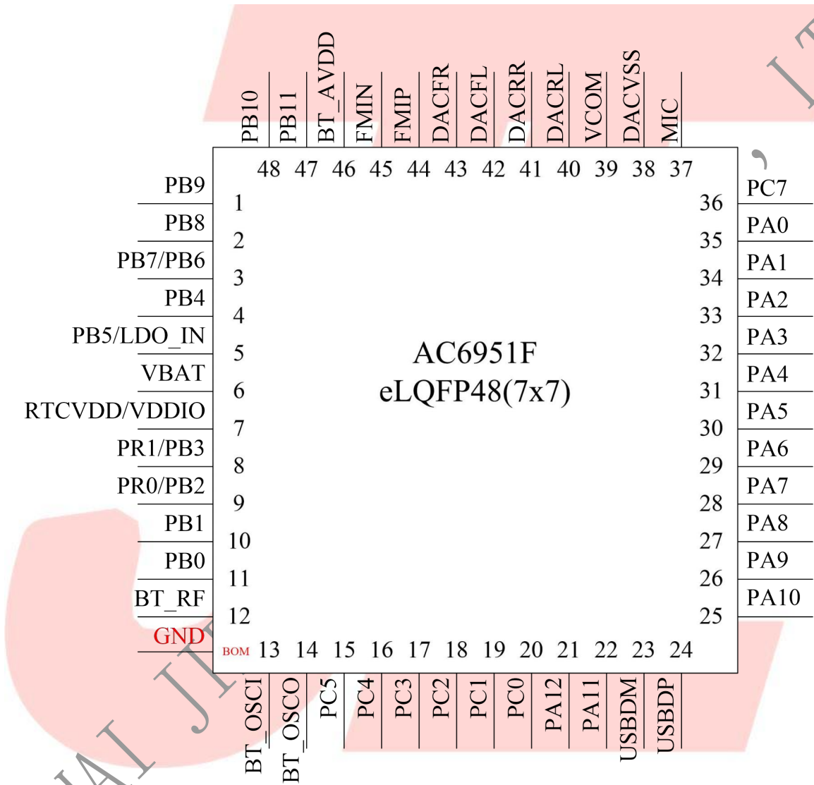
Figure 1-1 AC6951F_eLQFP48 Package Diagram
