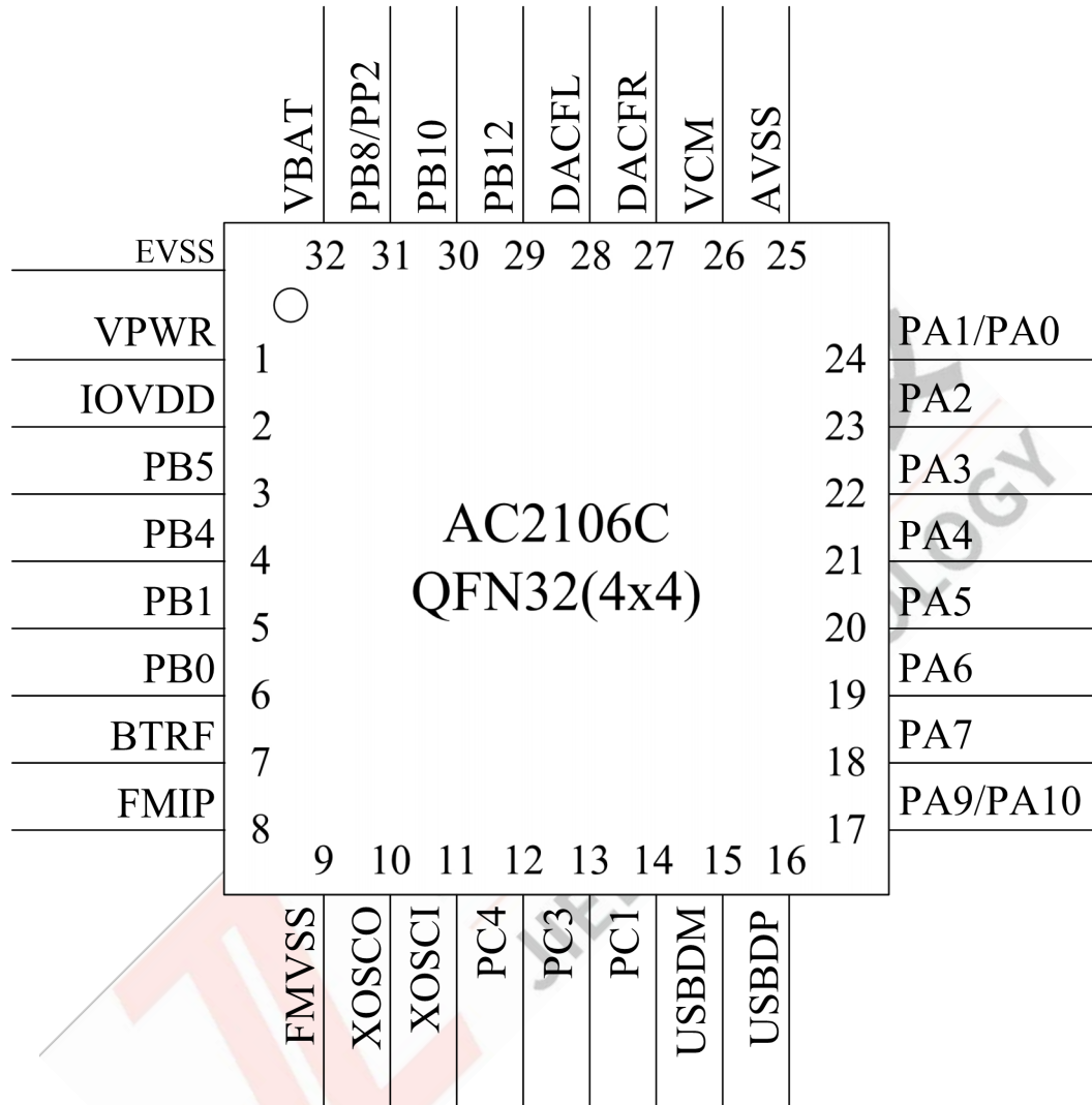
Figure 2-1 AC2106C Pin Assignment
