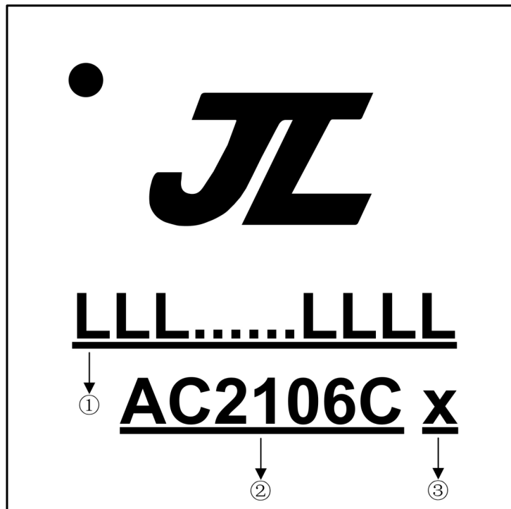
Figure 5-1 AC2106C Package Outline
