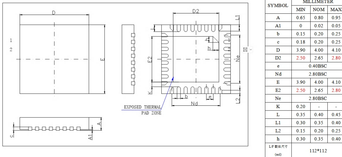
Figure 4-1 AC2106C Package
