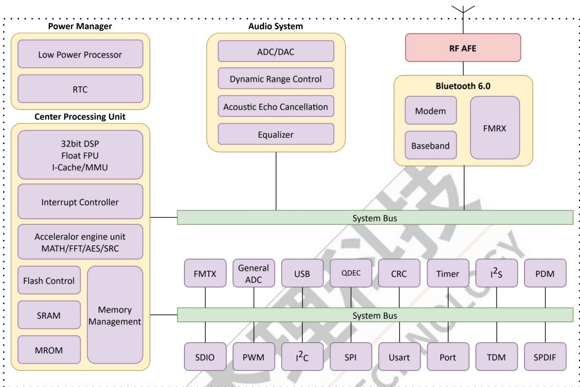
Figure 1-1 AC2106C Block Diagram
