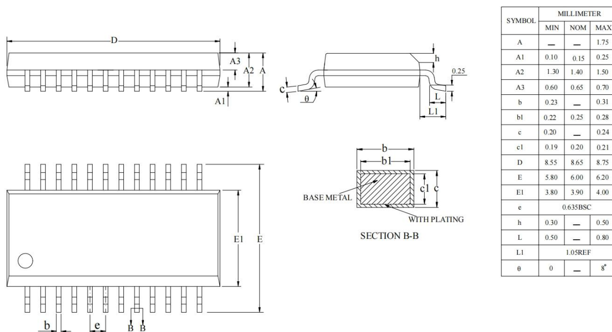
Figure 4-1 AC2105E Package
