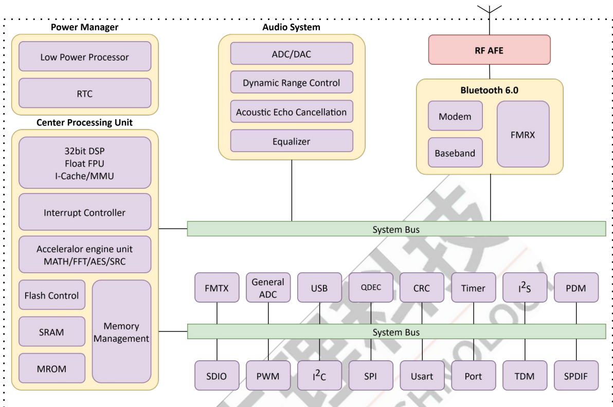
Figure 1-1 AC2105E Block Diagram
