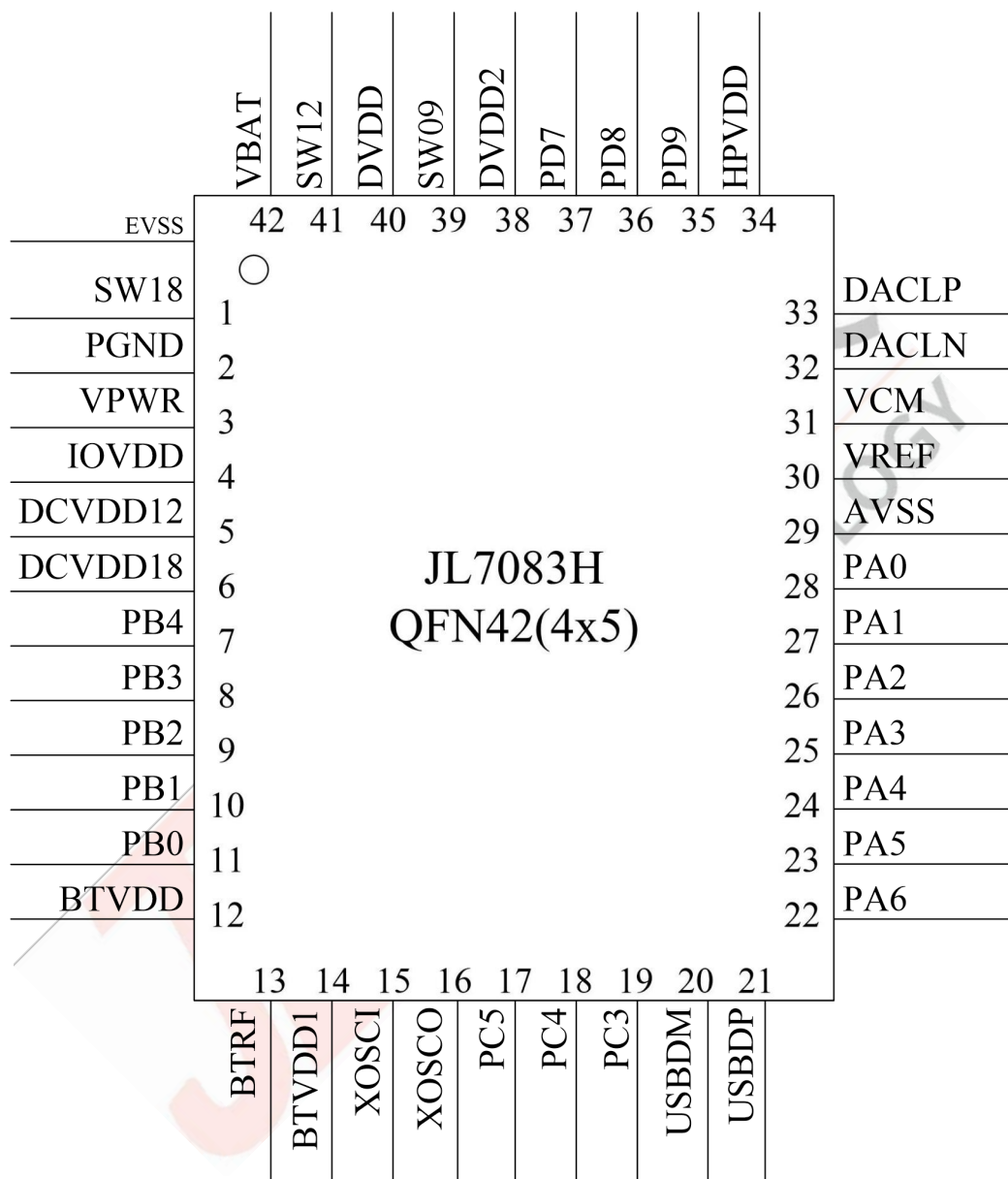
Figure 2-1 JL7083H Pin Assignment
