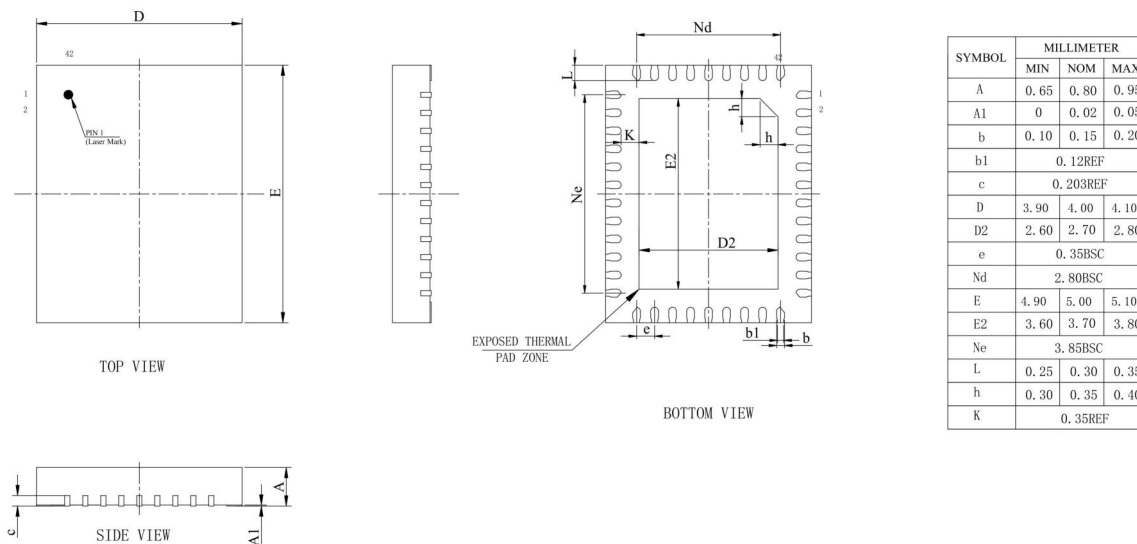
Figure 4-1 JL7083H Package
