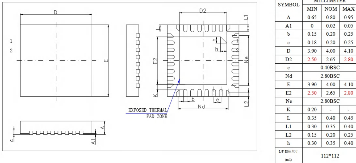
Figure 4-1 AW366A Package
