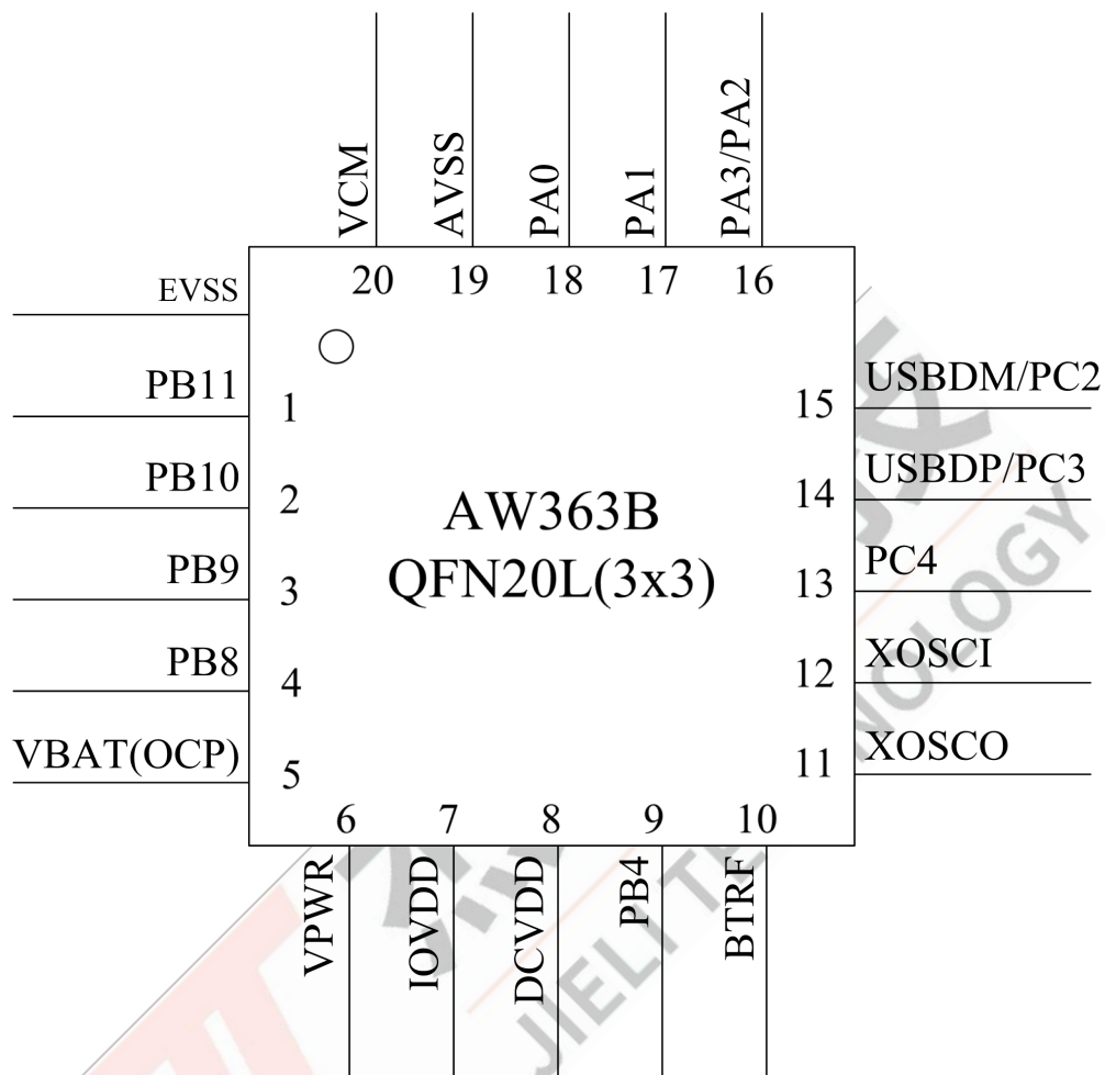
Figure 2-1 AW363B Pin Assignment
