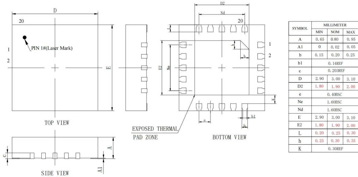
Figure 4-1 AW363B Package
