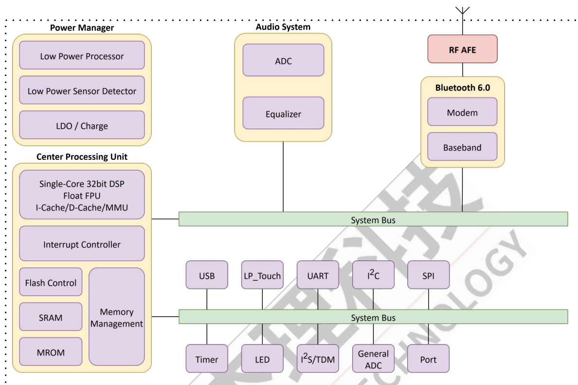
Figure 1-1 AW363B Block Diagram
