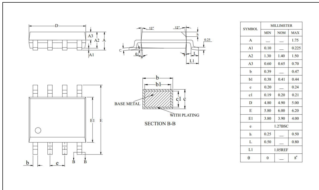
Figure 4-1 AW338A Package
