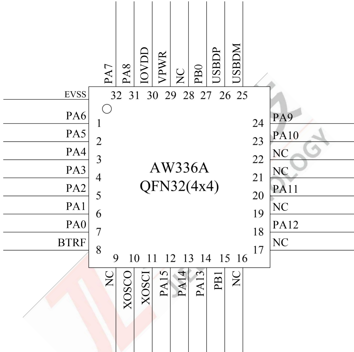
Figure 2-1 AW336A Pin Assignment
