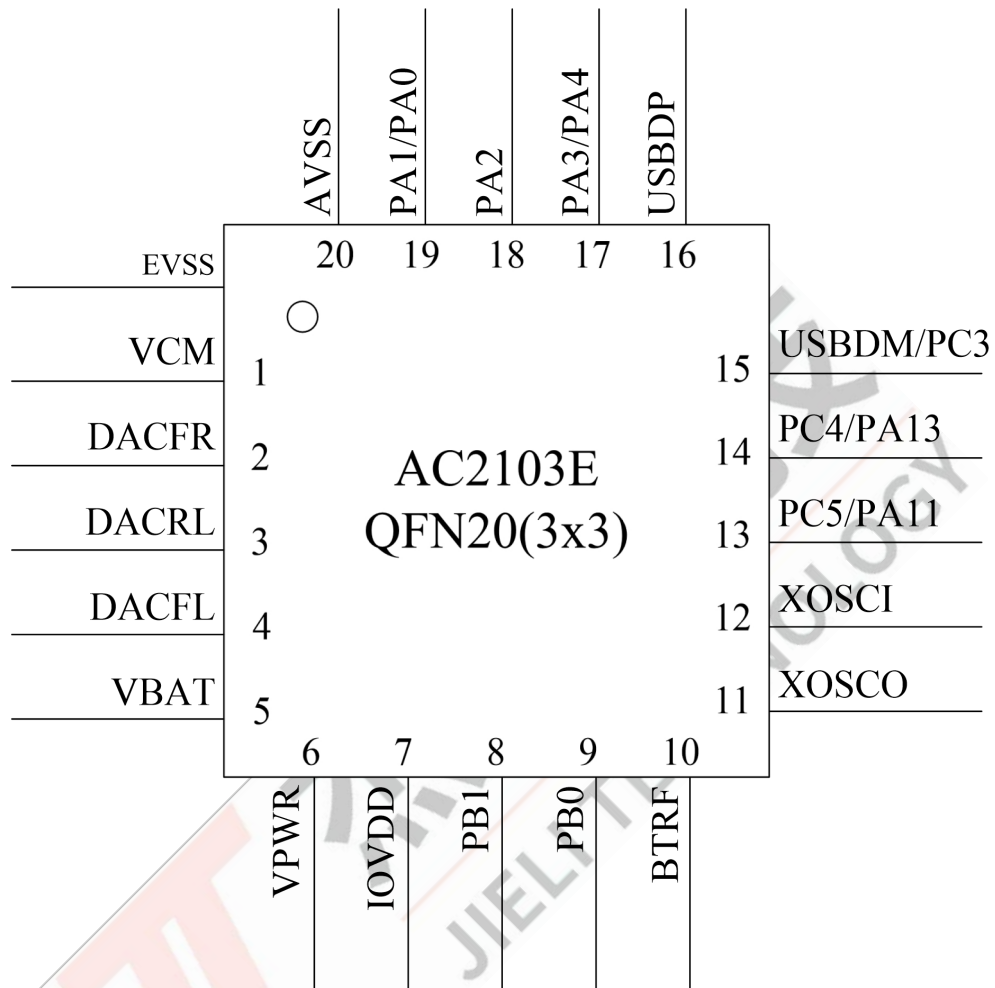
Figure 2-1 AC2103E Pin Assignment
