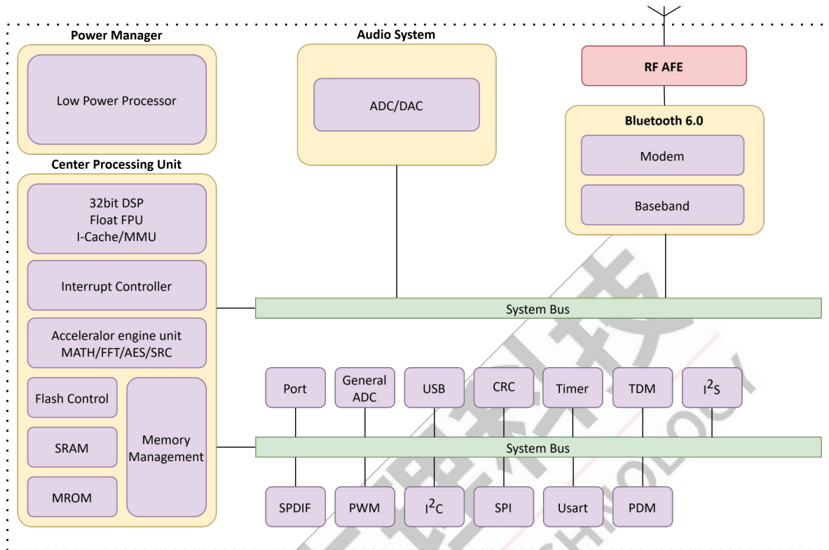
Figure 1-1 AC2103E Block Diagram
