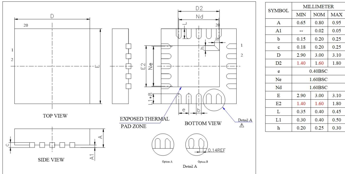
Figure 4-1 AC2103E Package
