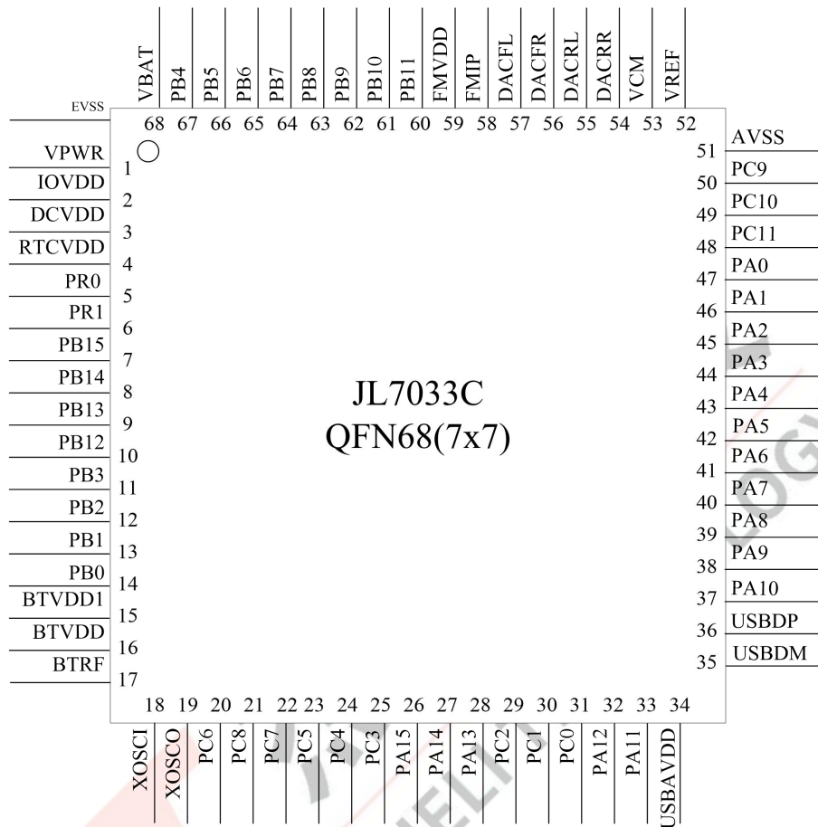
Figure 2-1-1 JL7033C Pin Assignment
