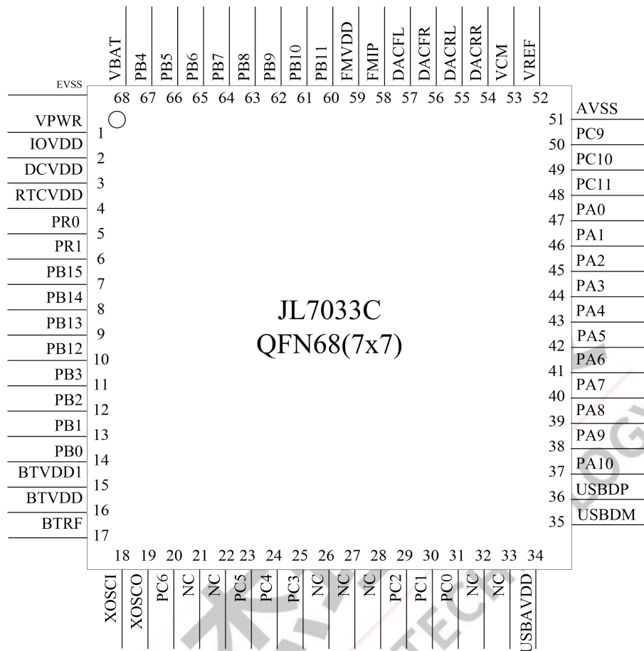
Figure 2-1-2 JL7033C(built-in PSRAM) Pin Assignment
