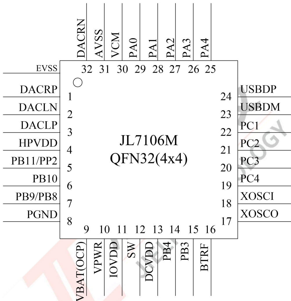
Figure 2-1 JL7106M Pin Assignment
