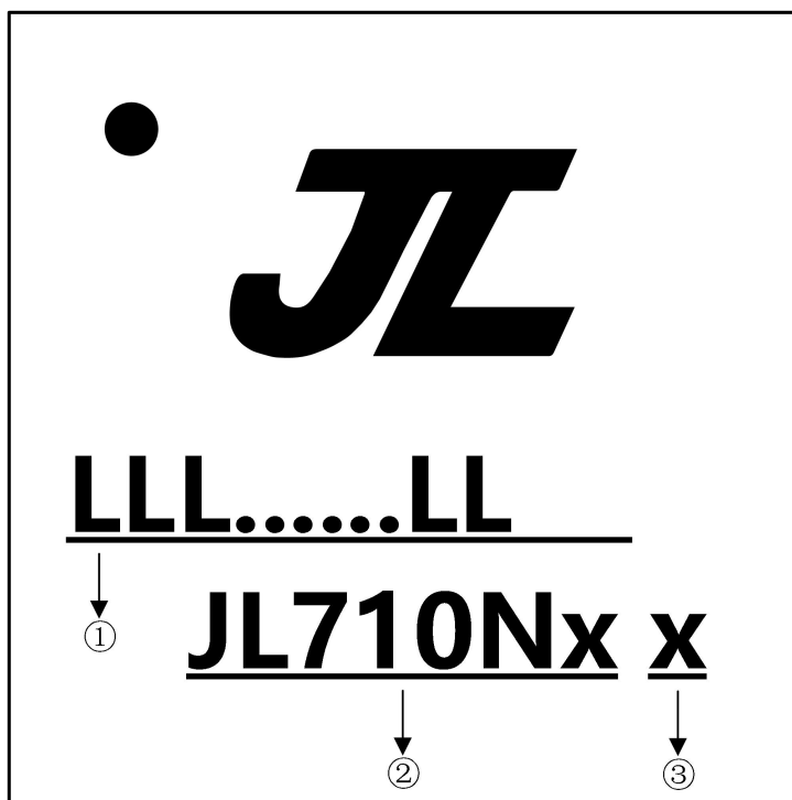
Figure 5-1 JL7106M Package Outline
