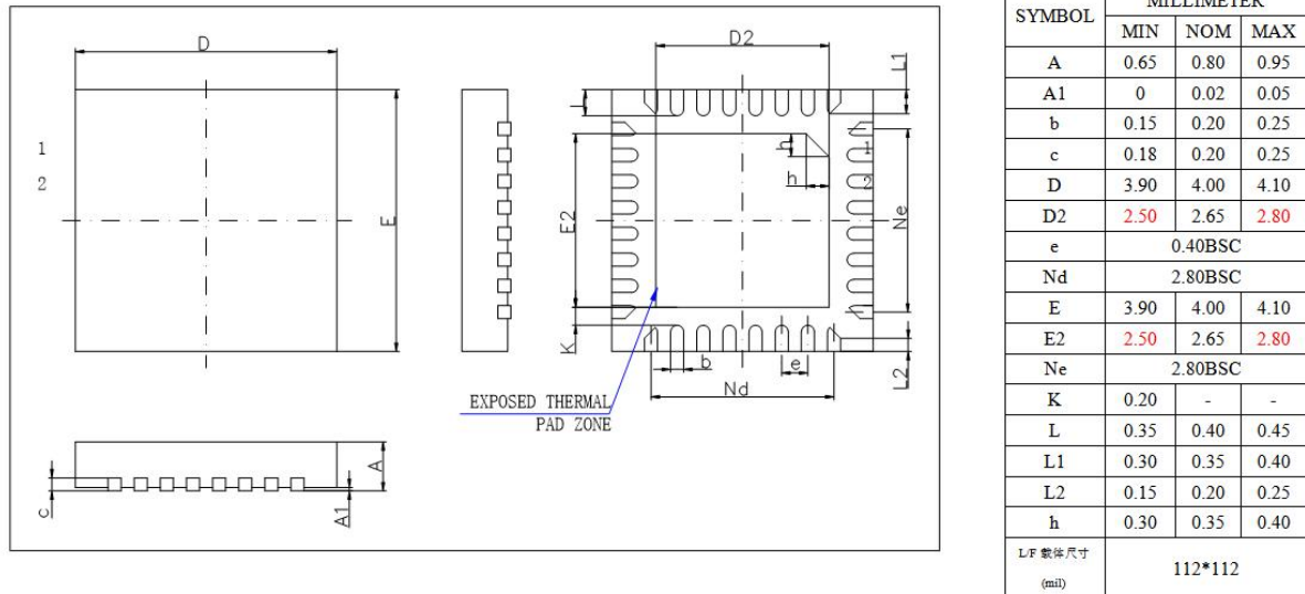
Figure 4-1 JL7106M Package
