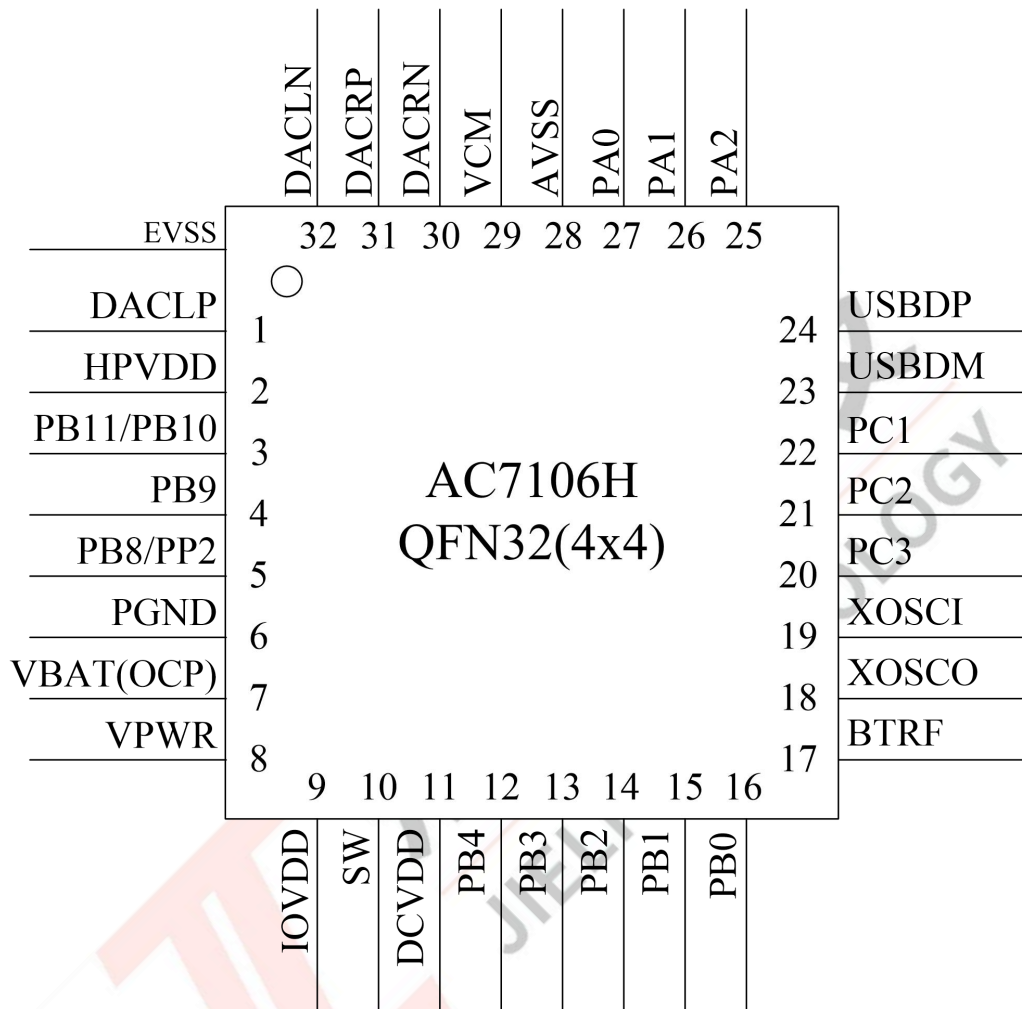
Figure 2-1 AC7106H Pin Assignment
