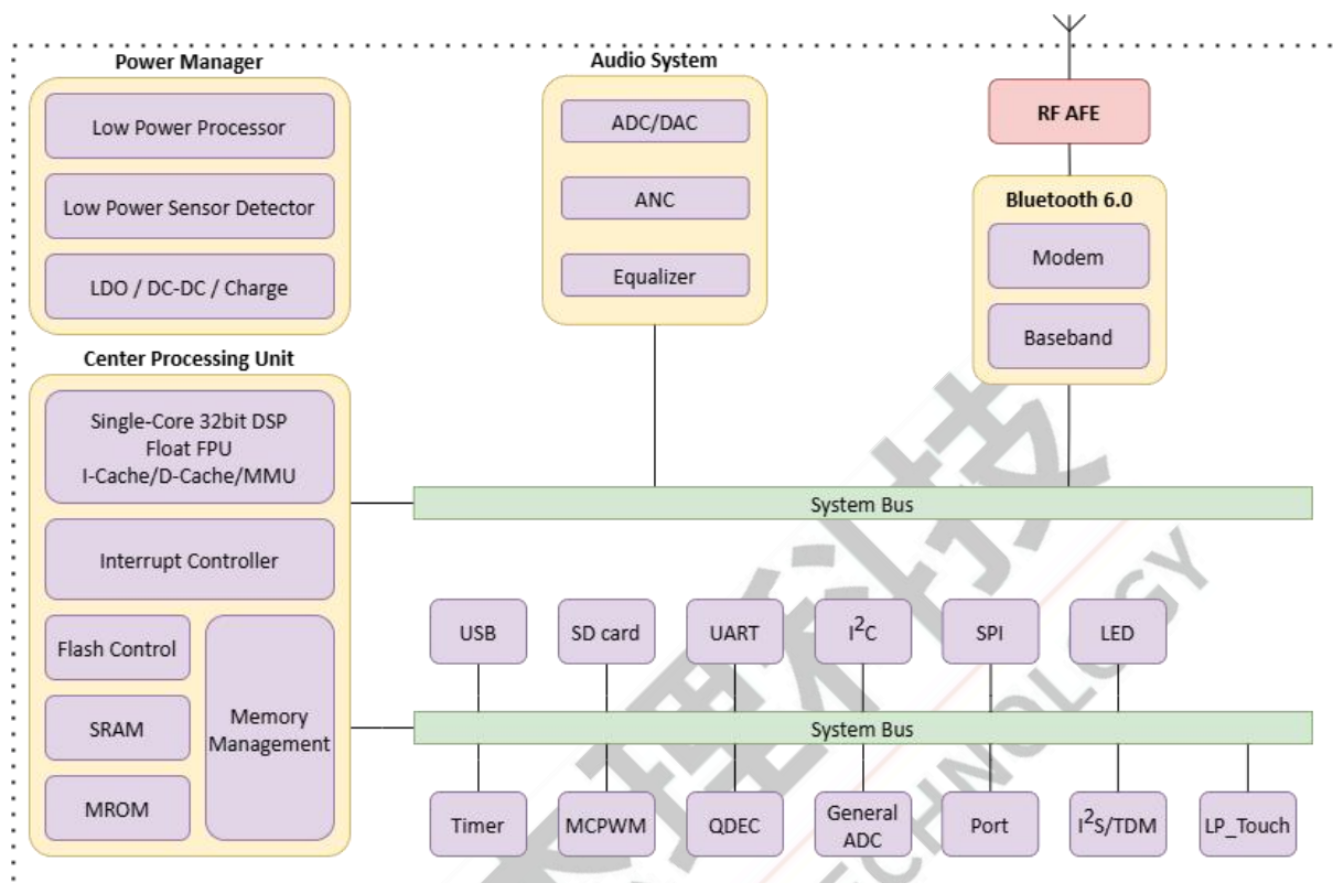
Figure 1-1 AC7106H Block Diagram
