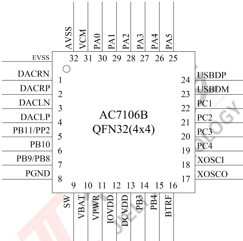
Figure 2-1 AC7106B Pin Assignment
