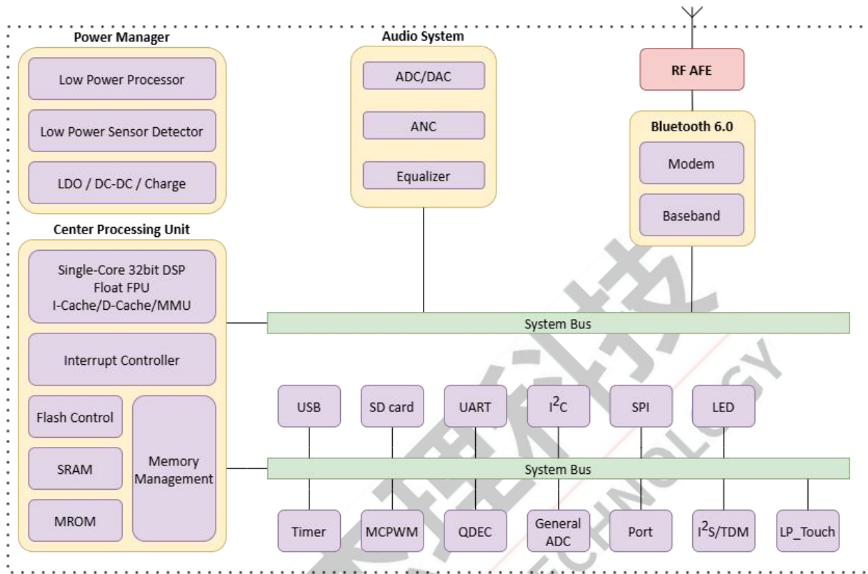
Figure 1-1 AC7106B Block Diagram
