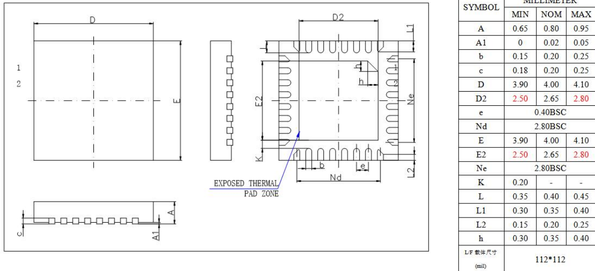
Figure 4-1 AC7106A Package
