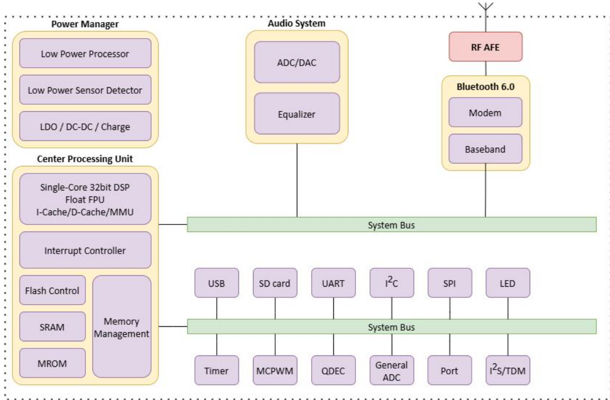
Figure 1-1 AC7103C Block Diagram
