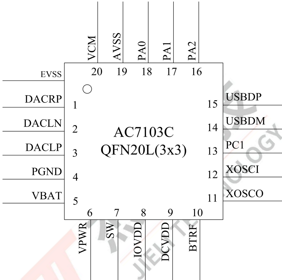
Figure 2-1 AC7103C Pin Assignment
