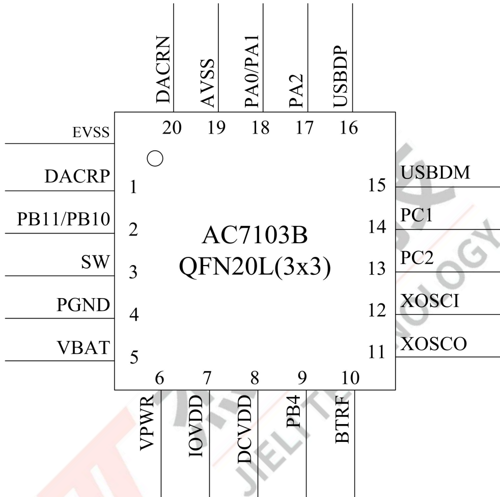
Figure 2-1 AC7103B Pin Assignment
