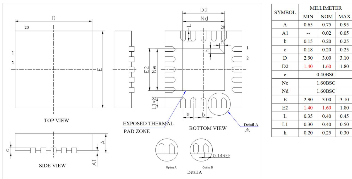
Figure 4-1 AW309A Package
