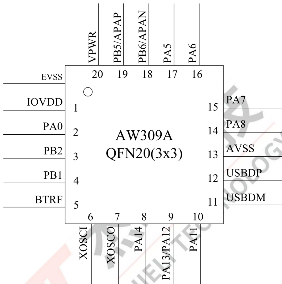
Figure 2-1 AW309A Pin Assignment
