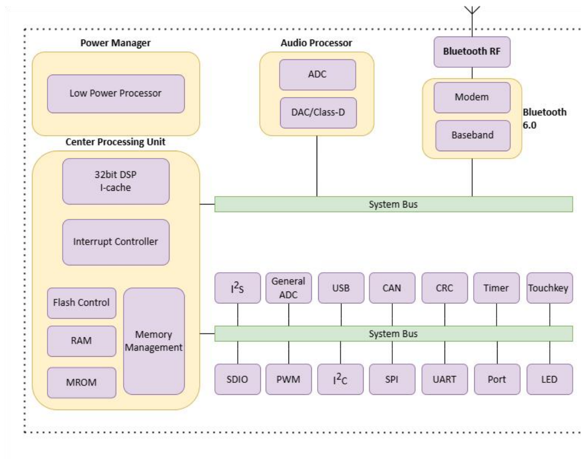
Figure 1-1 AW309A Block Diagram
