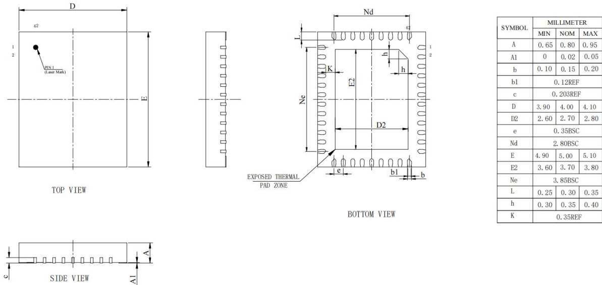
Figure 4-1 JL7094A Package
