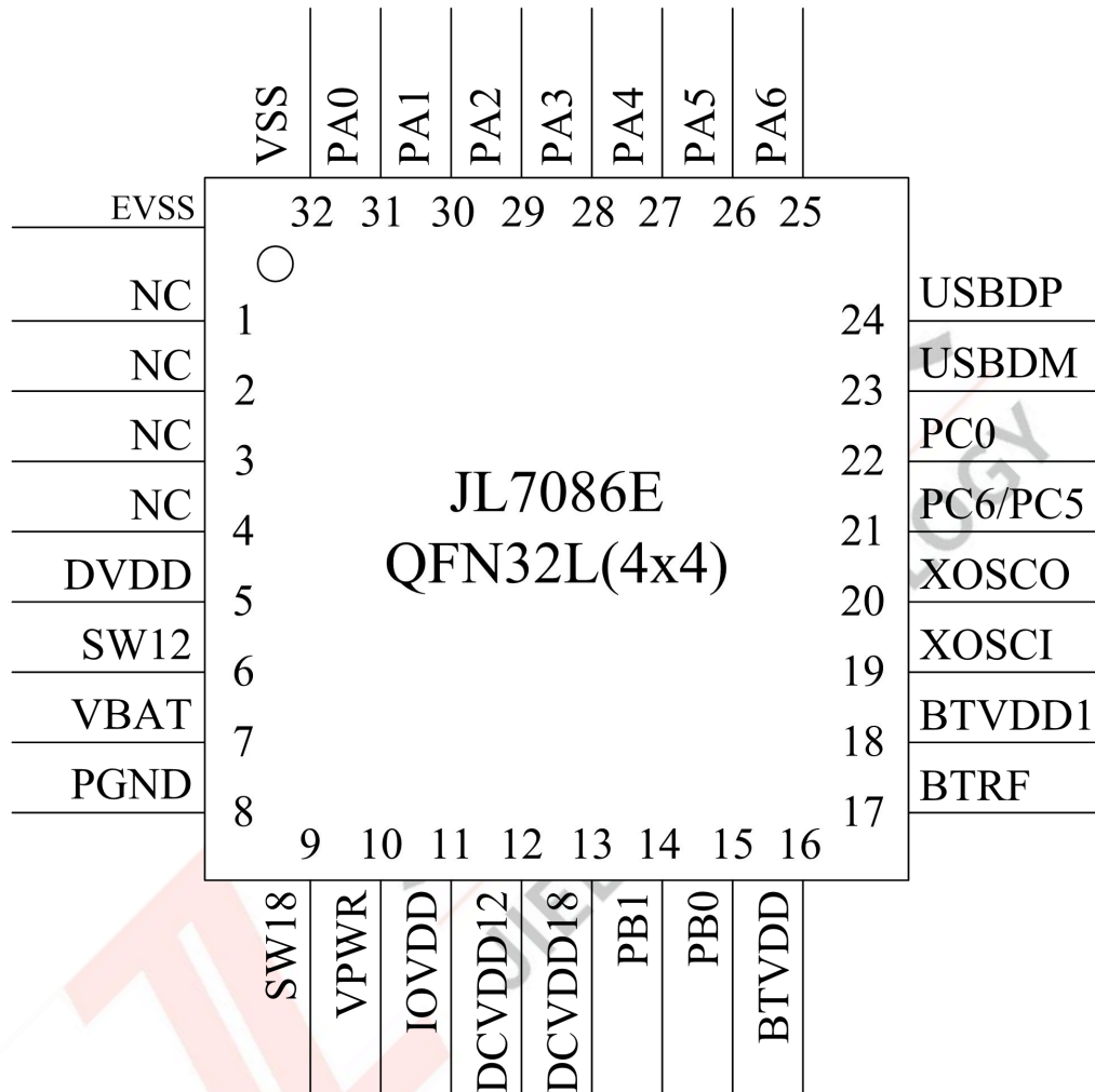
Figure 2-1 JL7086E Pin Assignment
