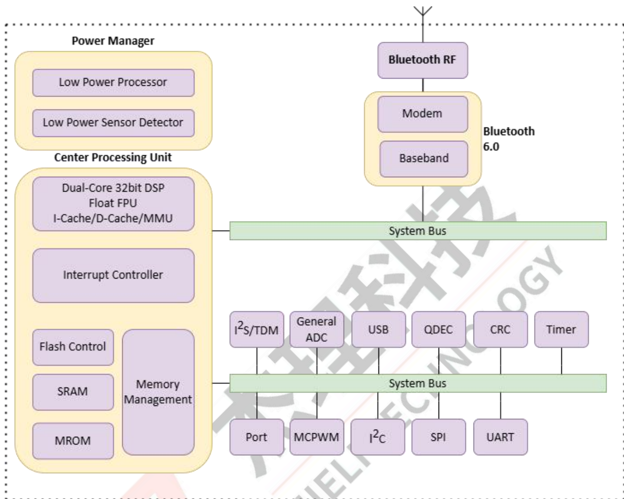
Figure 1-1 JL7086E Block Diagram
