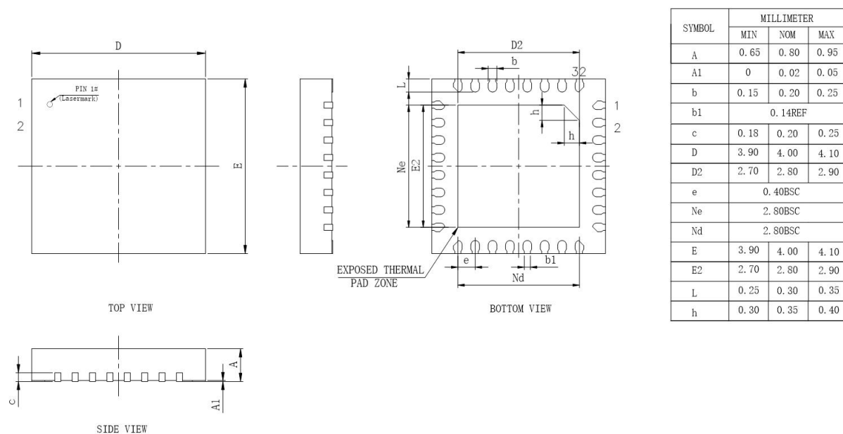
Figure 4-1 JL7086E Package
