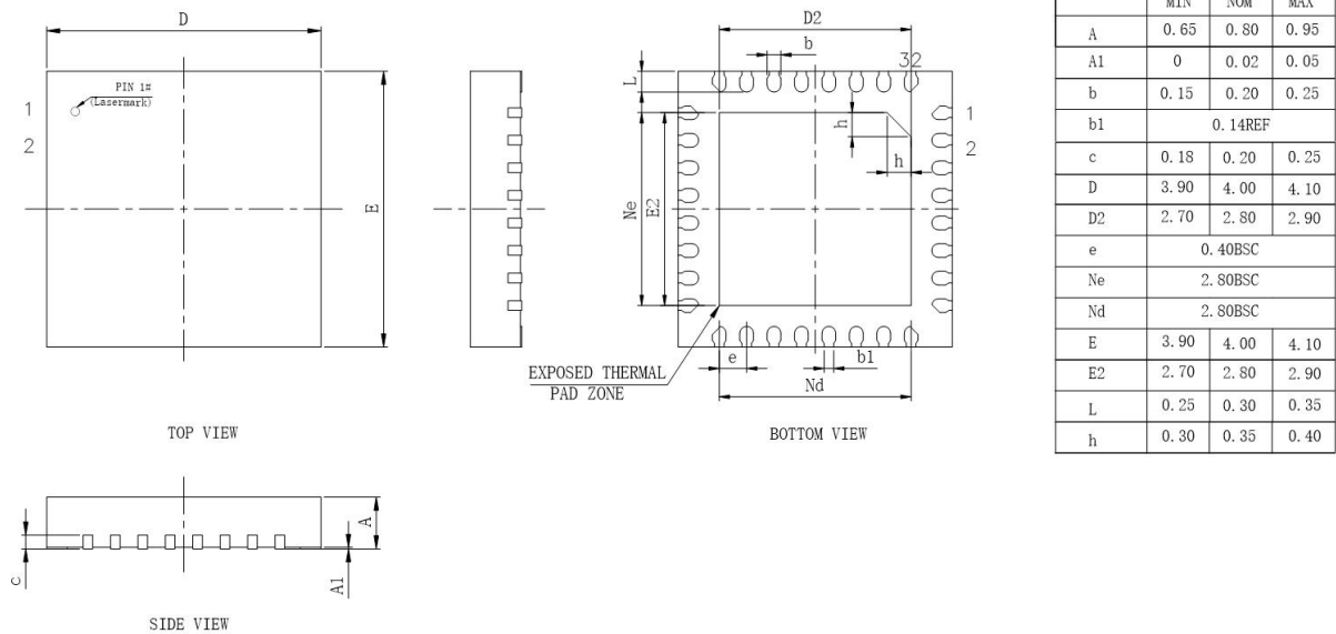
Figure 4-1 JL7086D Package
