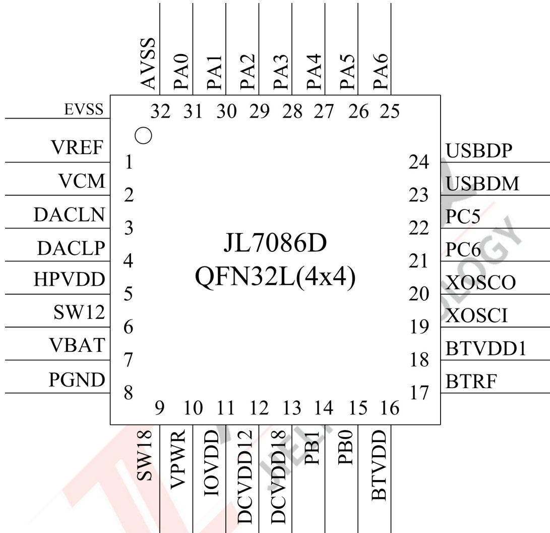
Figure 2-1 JL7086D Pin Assignment
