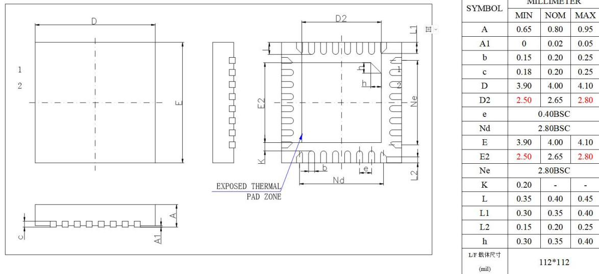
Figure 4-1 JL7096D Package
