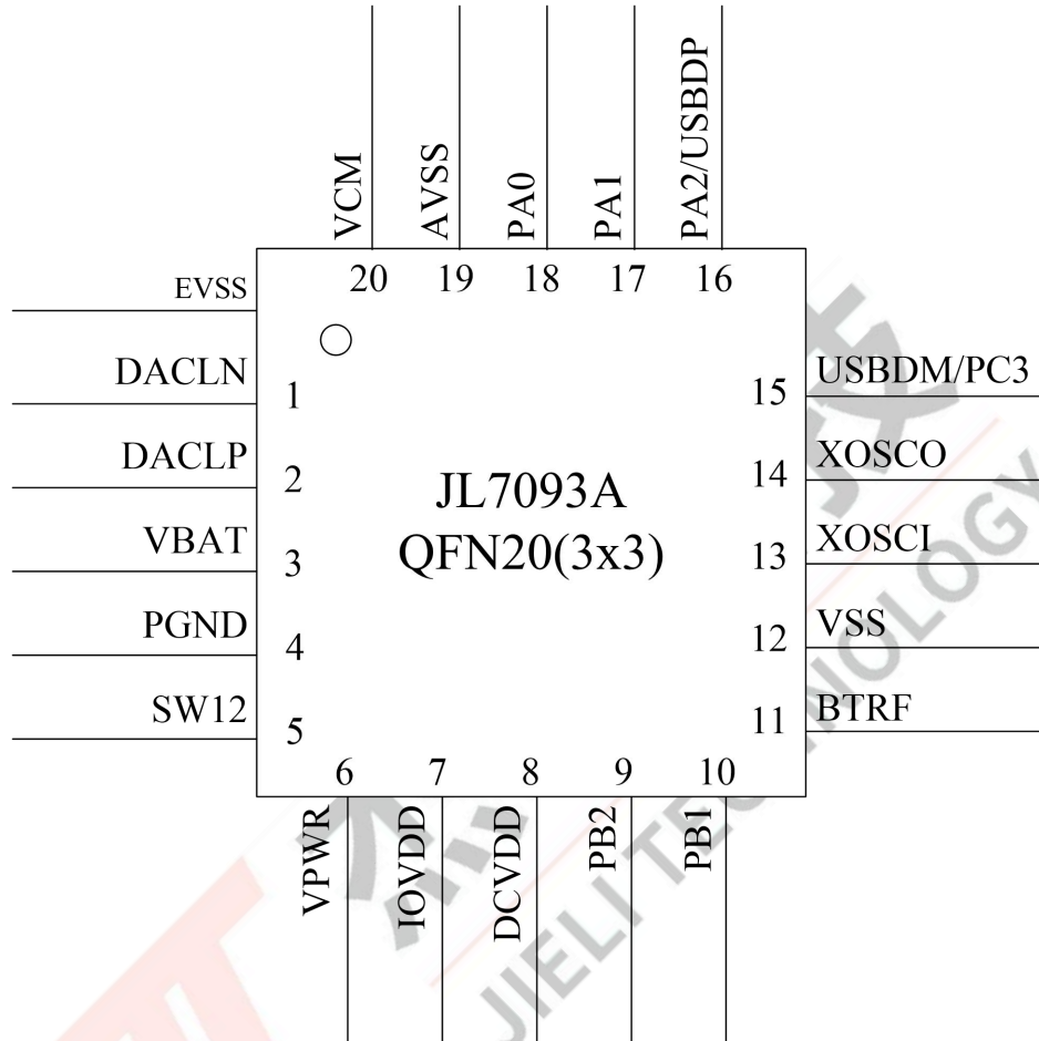
Figure 2-1 JL7093A Pin Assignment
