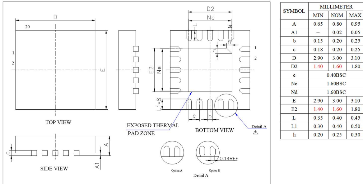
Figure 4-1 JL7093A Package
