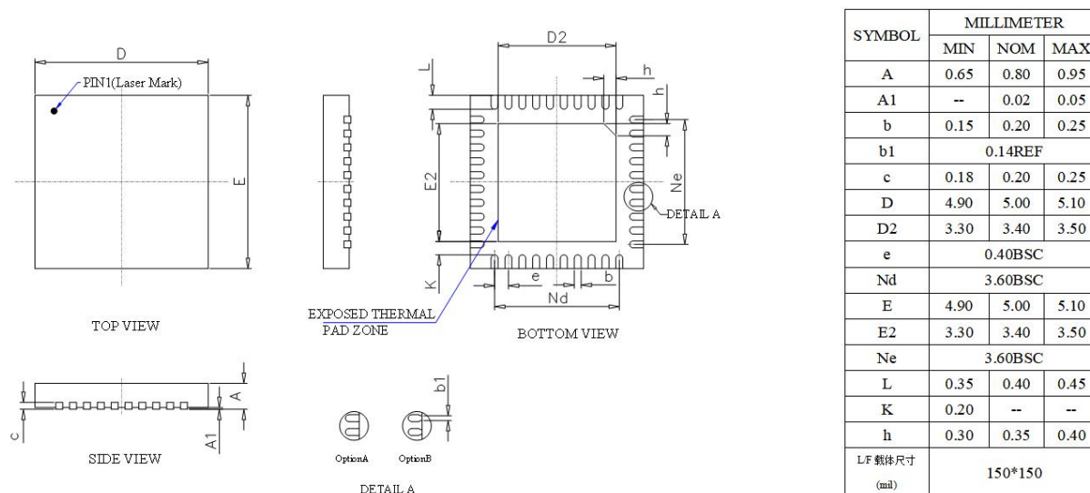
Figure 4-1 JL7032F Package
