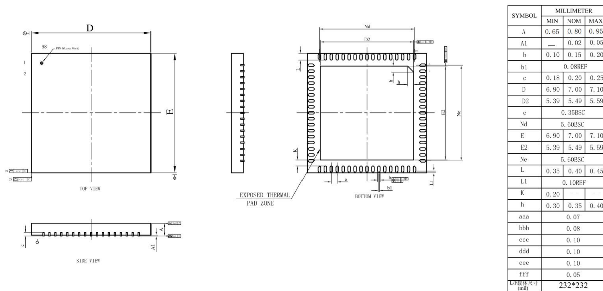
Figure 4-1 JL7033C Package
