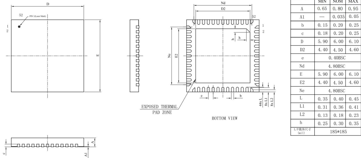
Figure 4-1 JL7034A Package
