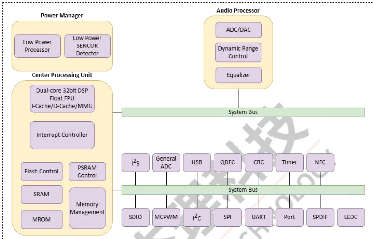
Figure 1-1 AC7036C Block Diagram
