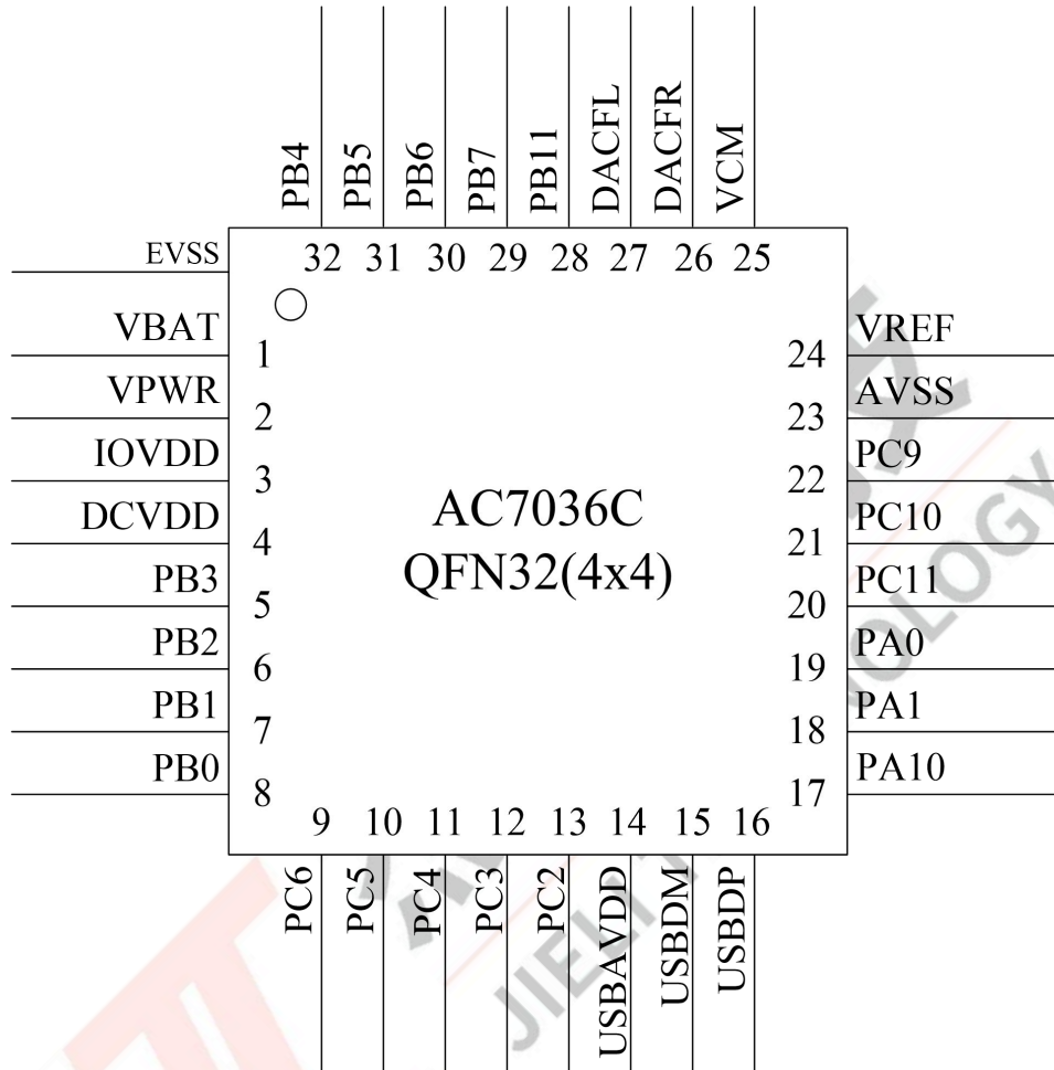
Figure 2-1 AC7036C Pin Assignment
