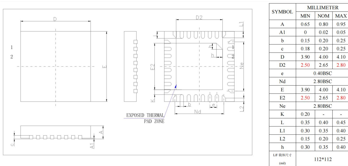
Figure 4-1 AC7036C Package
