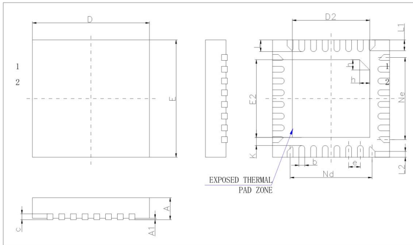
Figure 4-1 AC7106F Package
