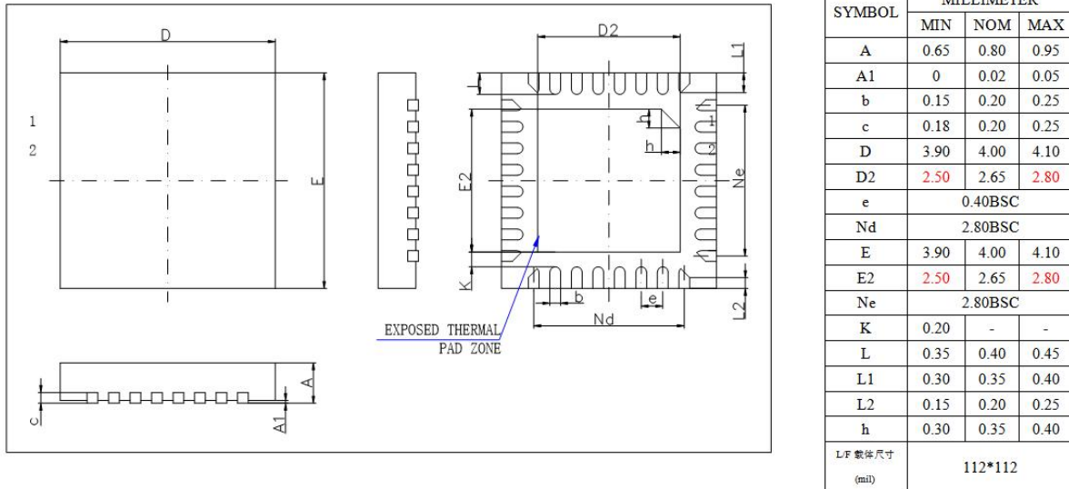
Figure 4-1 AC7106D Package
