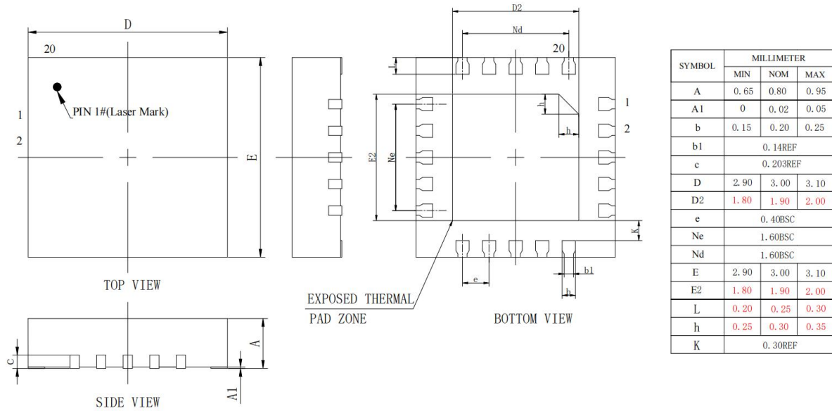
Figure 4-1 AC7103D Package
