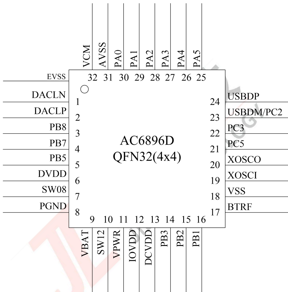
Figure 2-1 AC6896D Pin Assignment
