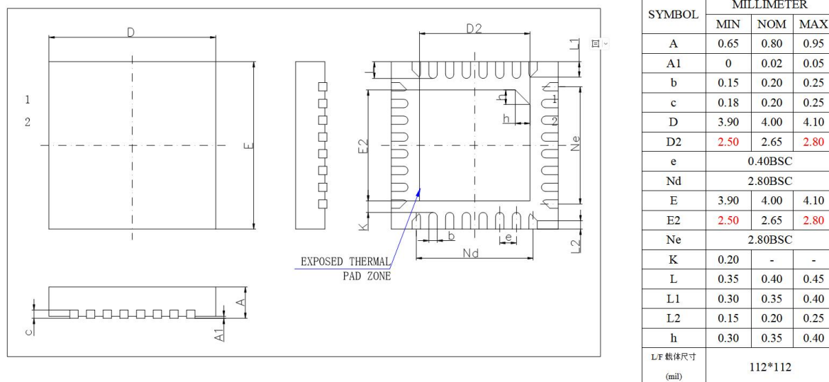
Figure 4-1 AC6896D Package
