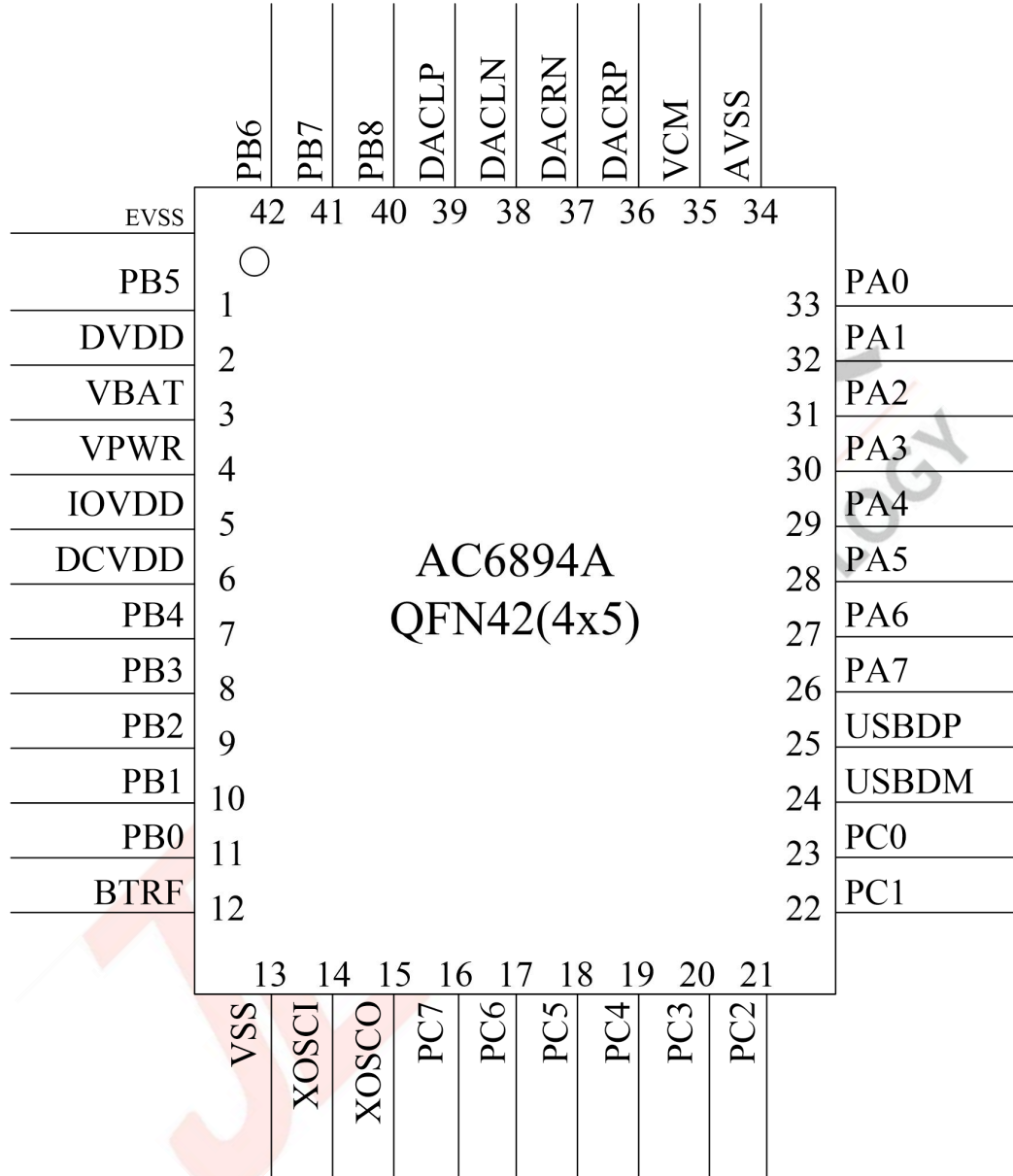
Figure 2-1 AC6894A Pin Assignment
