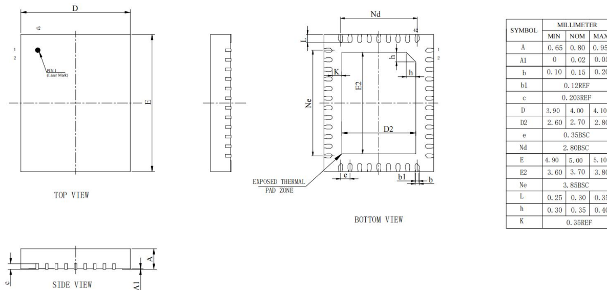
Figure 4-1 AC6894A Package
