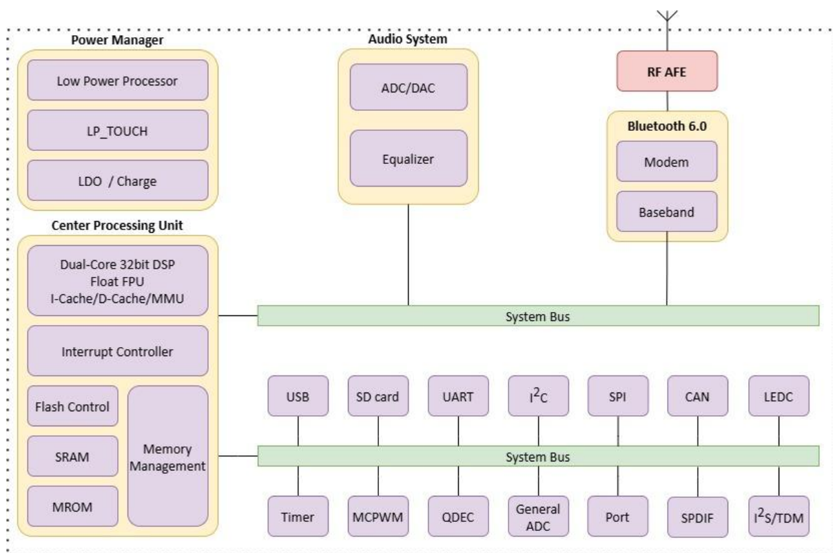
Figure 1-1 AC6894A Block Diagram
