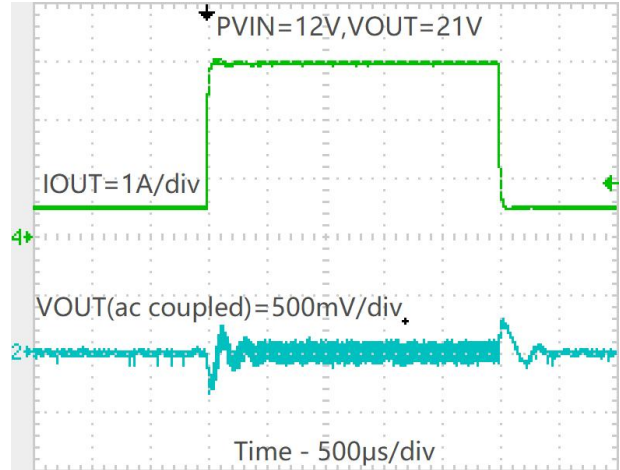
阶跃负载(PVIN=12V,VOUT=21V, IOUT=0.5A to 3A)
