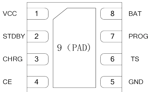
DFN2X2_8L
