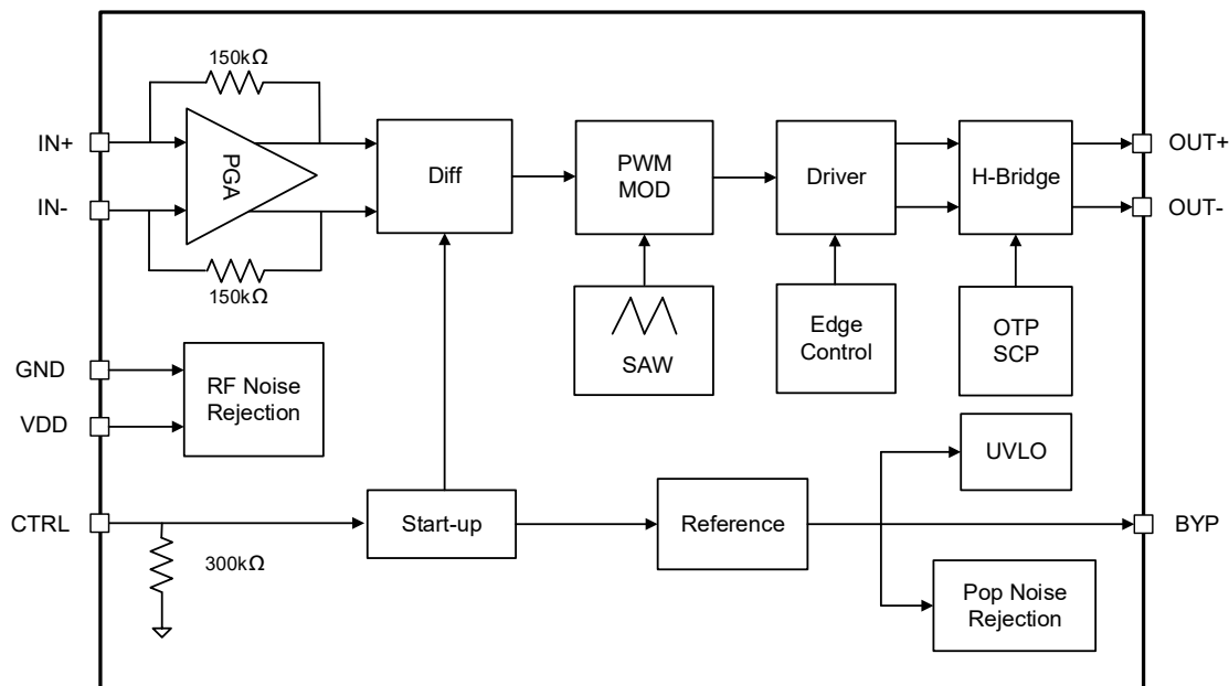
Figure 2: PF8009 Block Diagram
