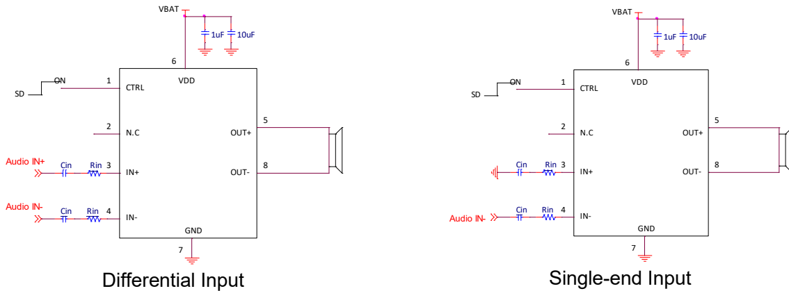
Figure 1. PF8009 Typical Application Circuit
