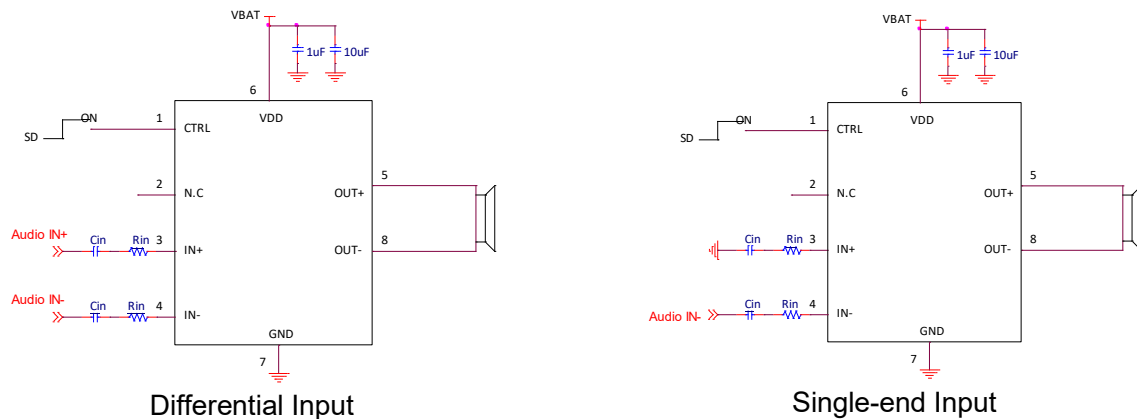
Figure 1. PF8008 Typical Application Circuit
