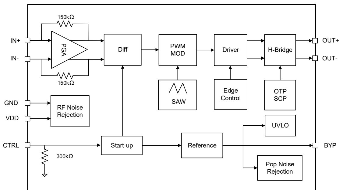
Figure 2: PF8008 Block Diagram
