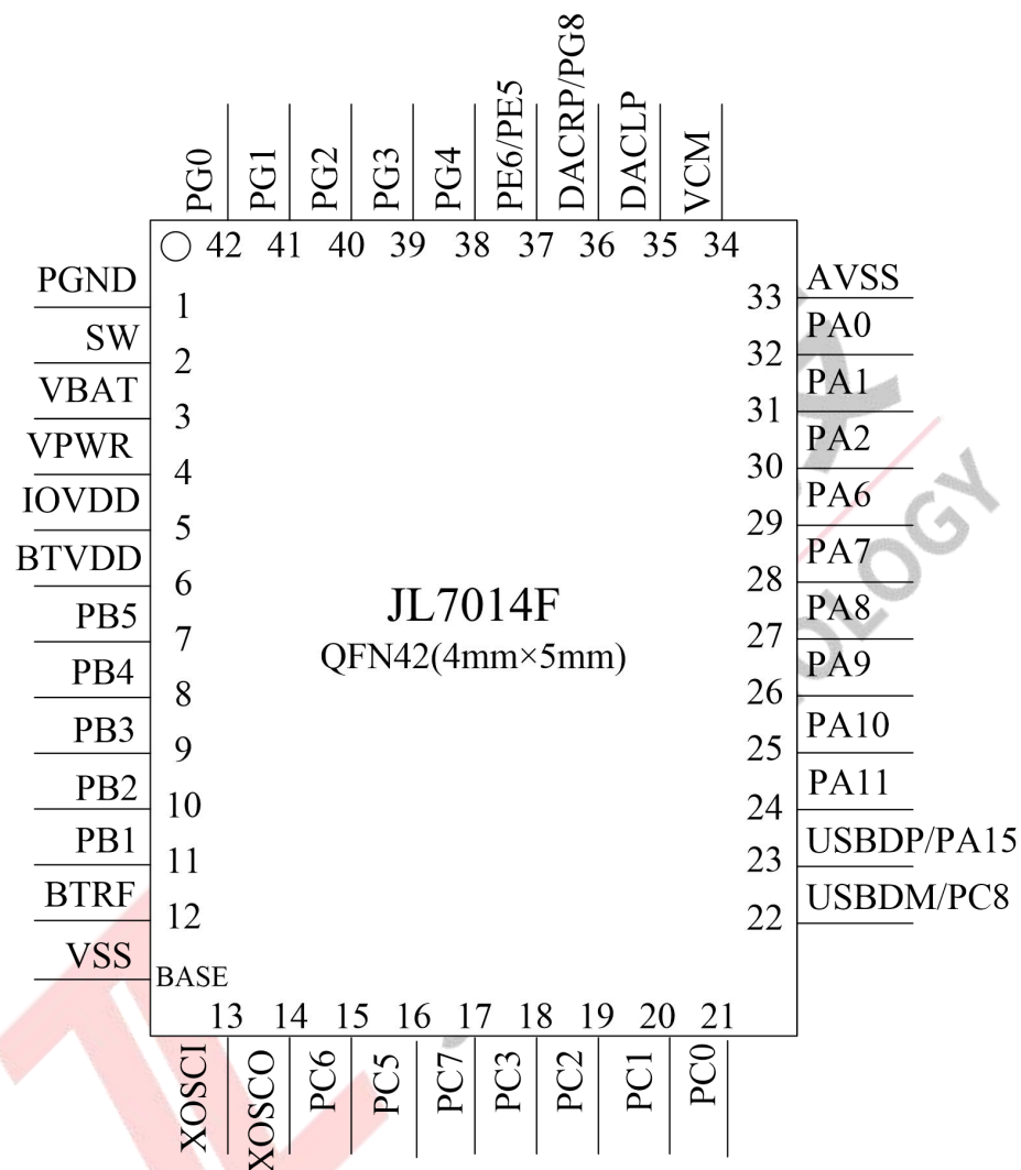
Figure 2-1 JL7014F Package Diagram
