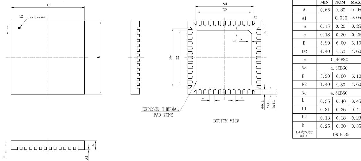
Figure 4-1 JL7012C Package
