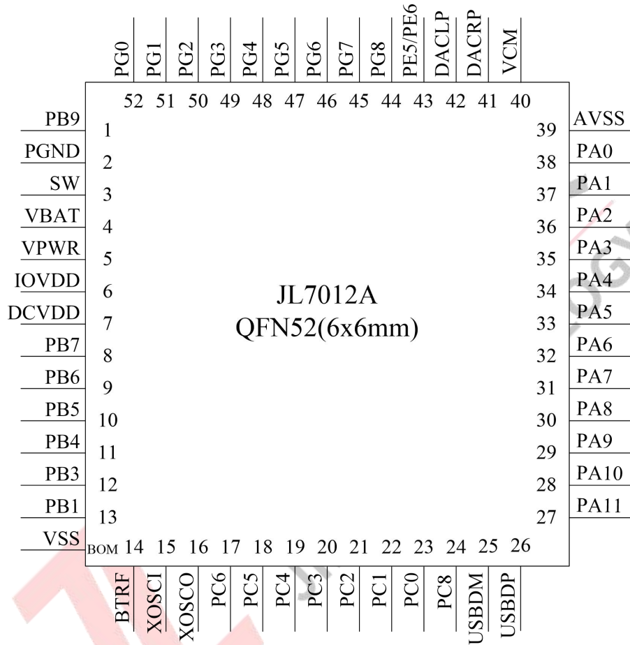
Figure 2-1 JL7012A Package Diagram
