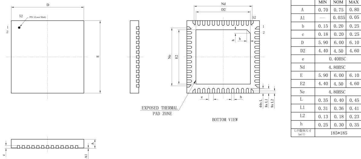
Figure 4-1 JL7012A Package
