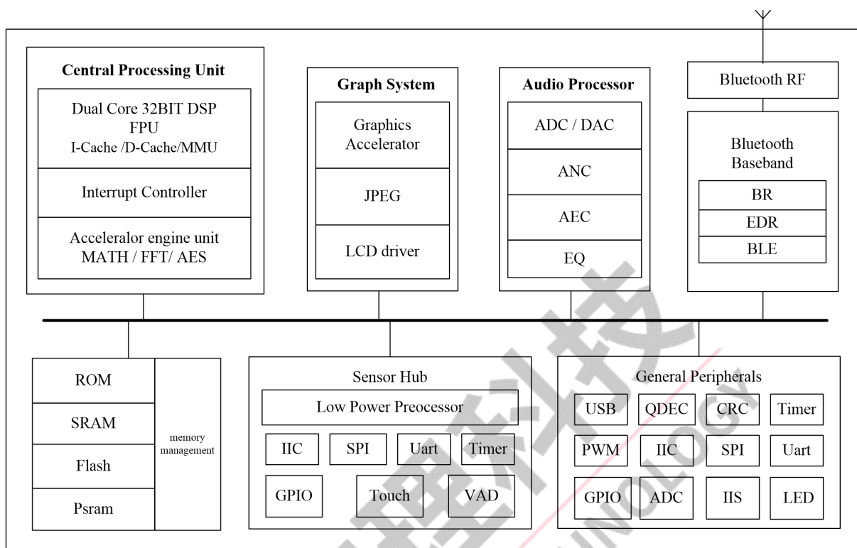
Figure 1-1 JL7012A Block Diagram
