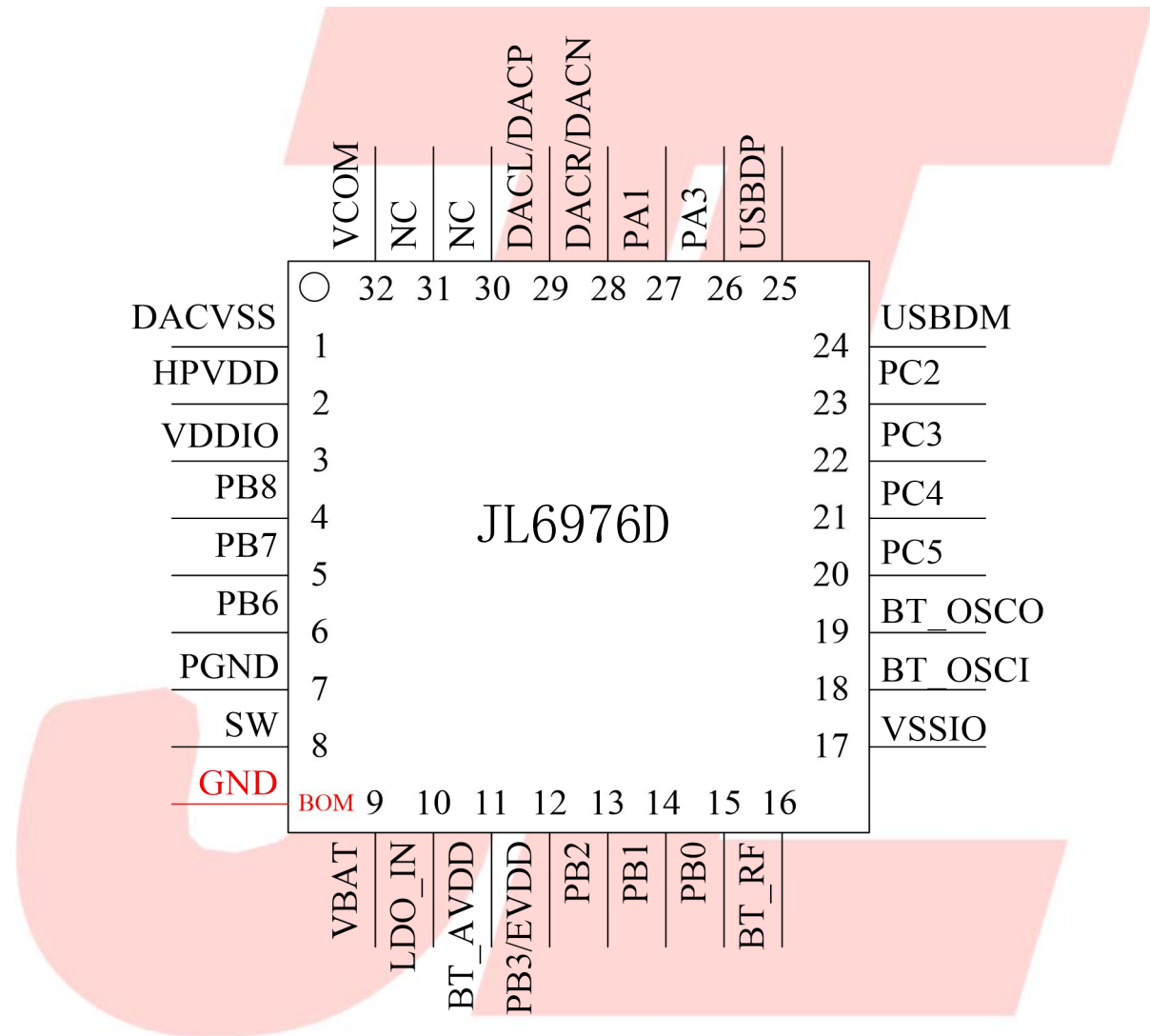
Figure 1-1 JL6976D Package Diagram
