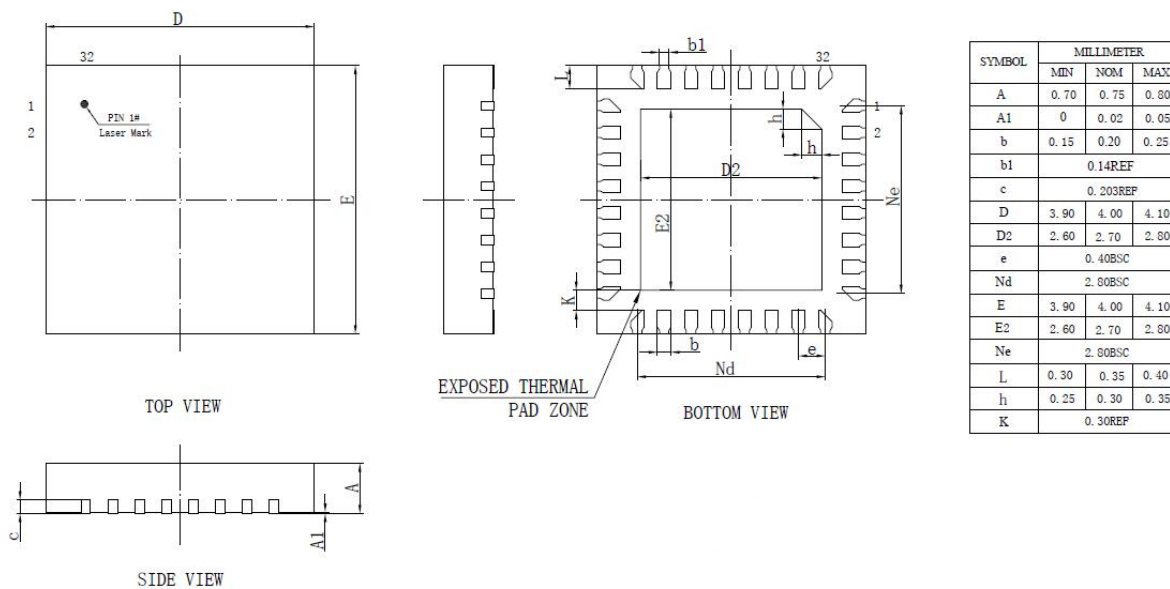
Figure 3-1 JL6976D Package
