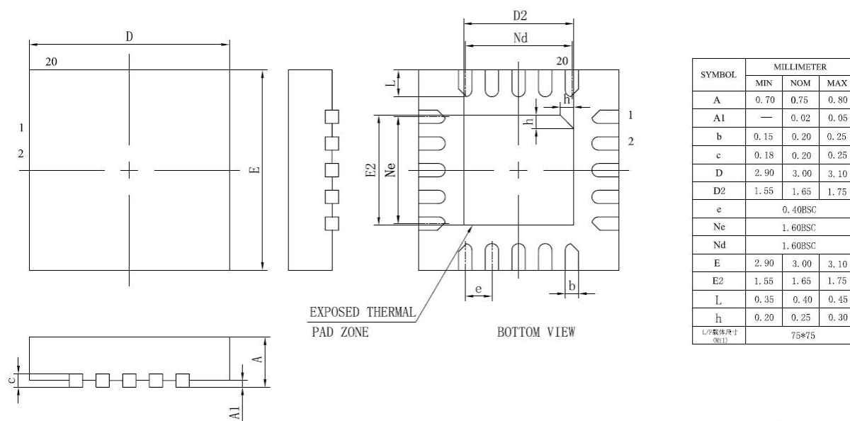
Figure 3-1 AD6973D Package
