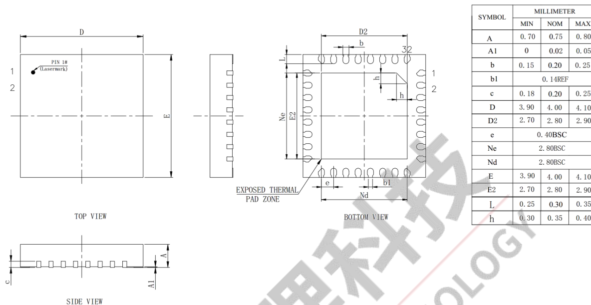
Figure 4-1 AC7076A Package
